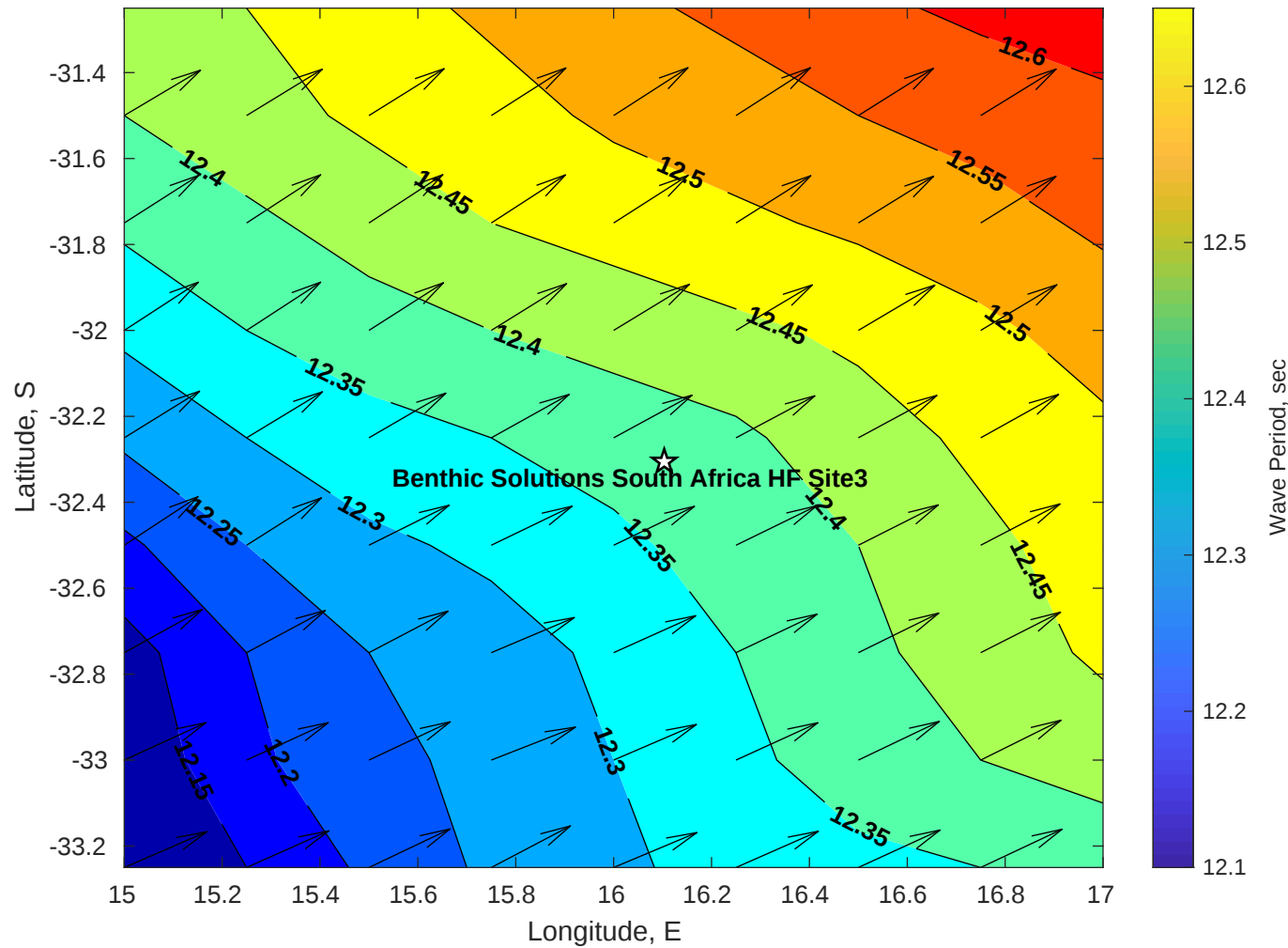
Wave Period (sec) for Benthic Solutions South Africa HF Site3 at 15-May-2025 09:00:00
