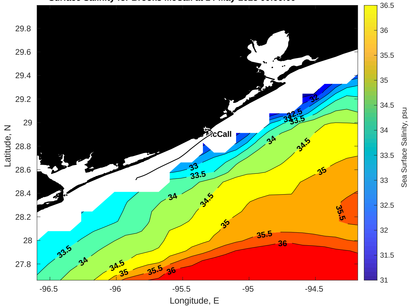
Surface Salinity for Brooks McCall at 14-May-2025 00:00:00
