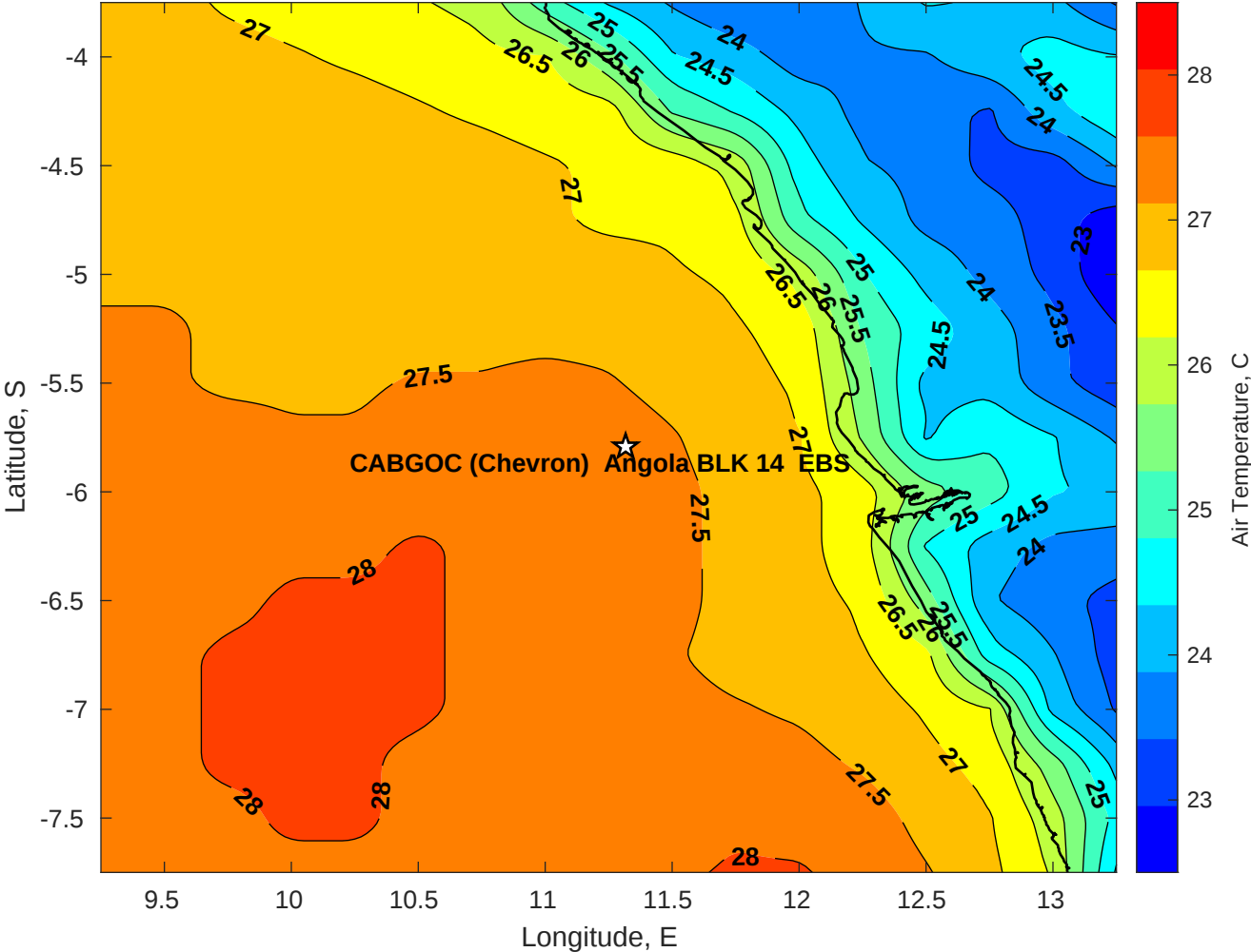
Air Temperature (C) for CABGOC (Chevron) Angola BLK 14 EBS at 15-May-2025
