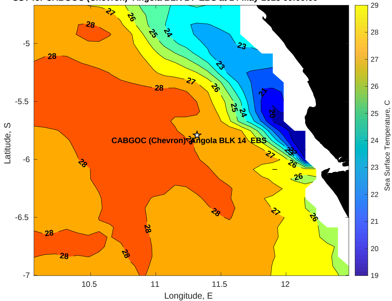
SST for CABGOC (Chevron) Angola BLK 14 EBS at 14-May-2025 00:00:00
