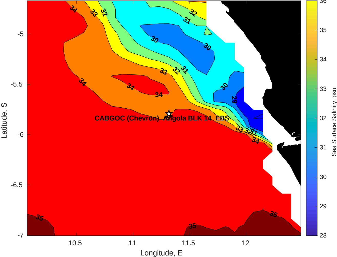
Surface Salinity for CABGOC (Chevron) Angola BLK 14 EBS at 14-May-2025 00:00:00
