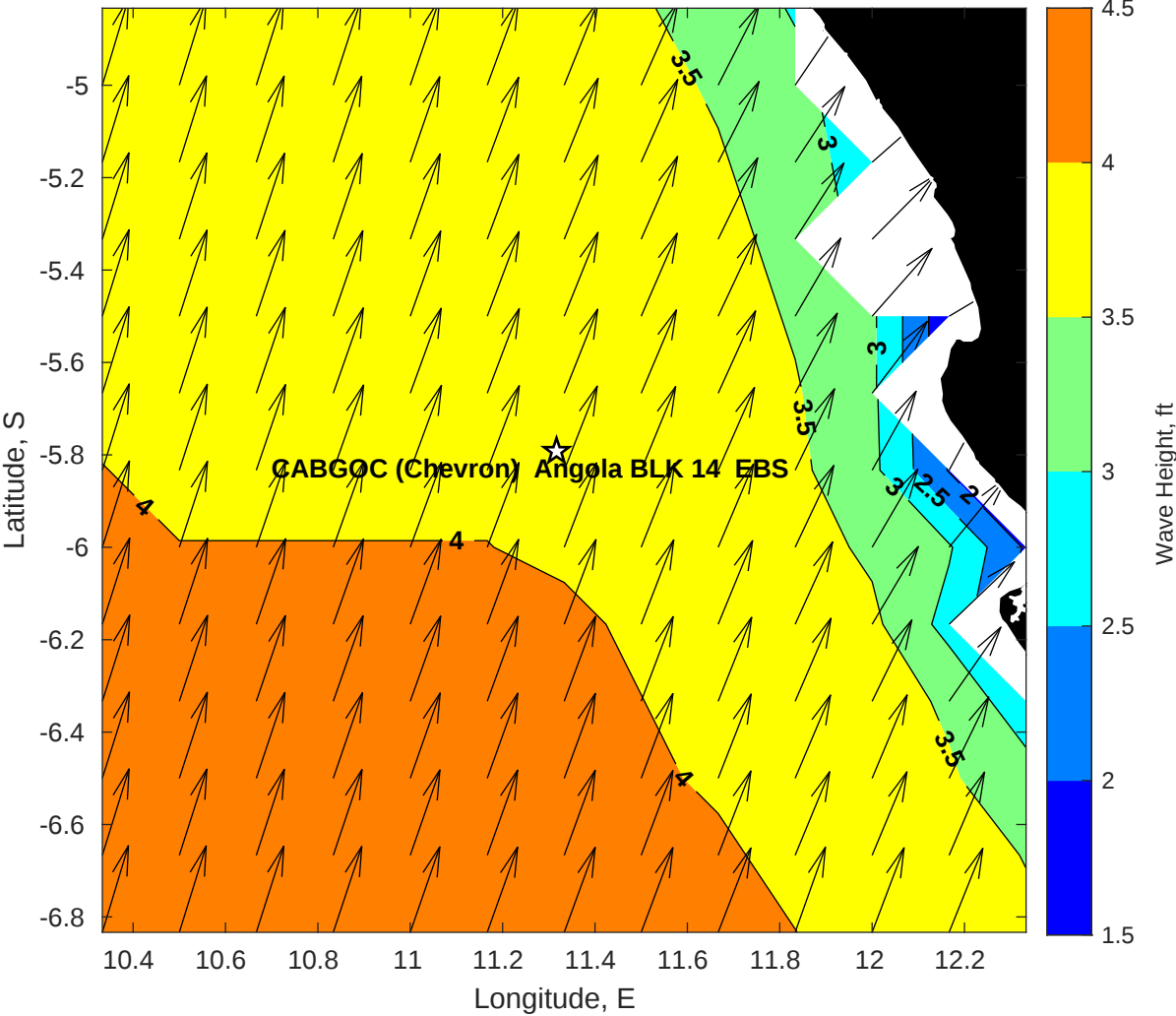
Wave Height (ft) for CABGOC (Chevron) Angola BLK 14 EBS at 15-May-2025 09:00:00
