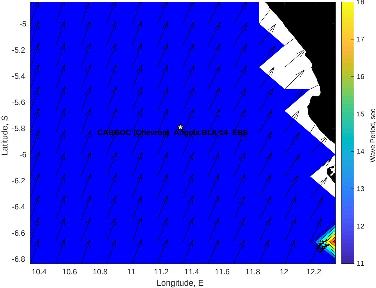
Wave Period (sec) for CABGOC (Chevron) Angola BLK 14 EBS at 15-May-2025 09:00:00
