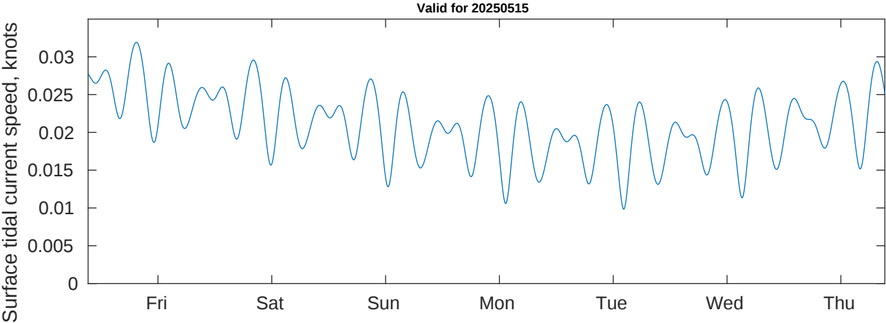
Tidal Currents and Heights for CABGOC (Chevron) Angola BLK 14 EBS at 20250515
