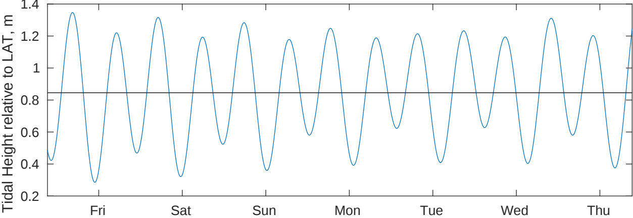
Tidal Currents and Heights for CABGOC (Chevron) Angola BLK 14 EBS at 20250515
