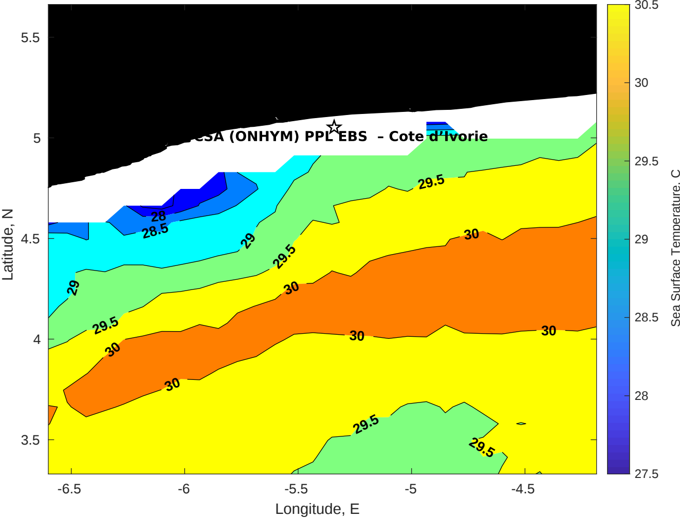
SST for CSA (ONHYM) PPL EBS - Cote d'Ivoire at 14-May-2025 00:00:00
