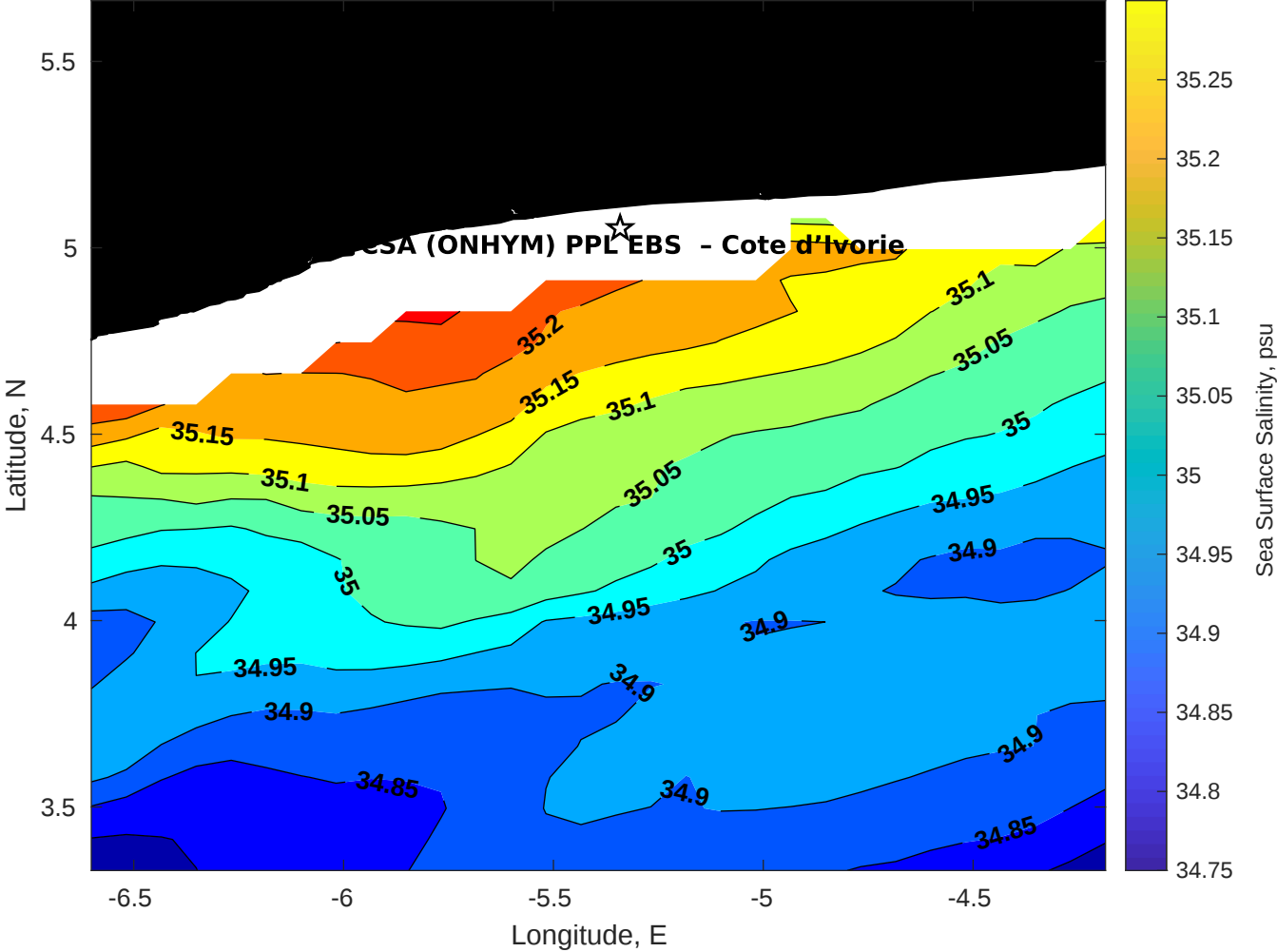
Surface Salinity for CSA (ONHYM) PPL EBS - Cote d'Ivoire at 14-May-2025 00:00:00
