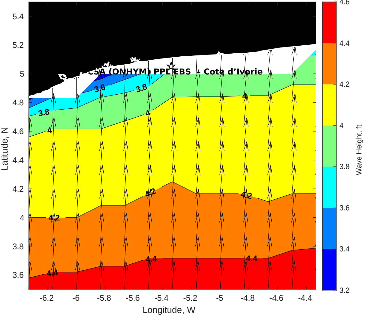
Wave Height (ft) for CSA (ONHYM) PPL EBS - Cote d'Ivoire at 15-May-2025 09:00:00
