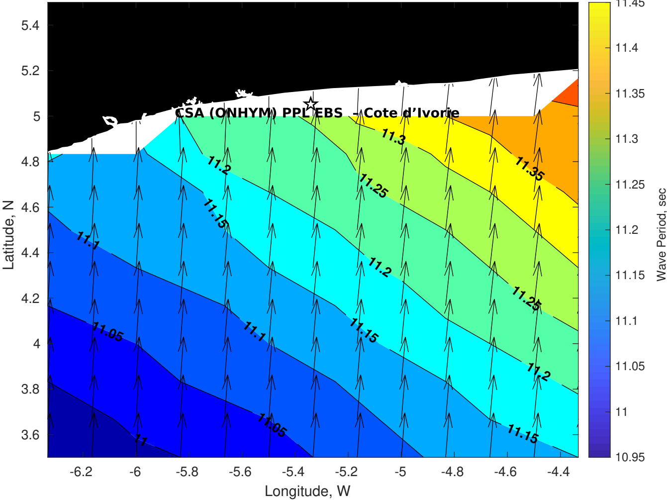
Wave Period (sec) for CSA (ONHYM) PPL EBS - Cote d'Ivoire at 15-May-2025 09:00:00
