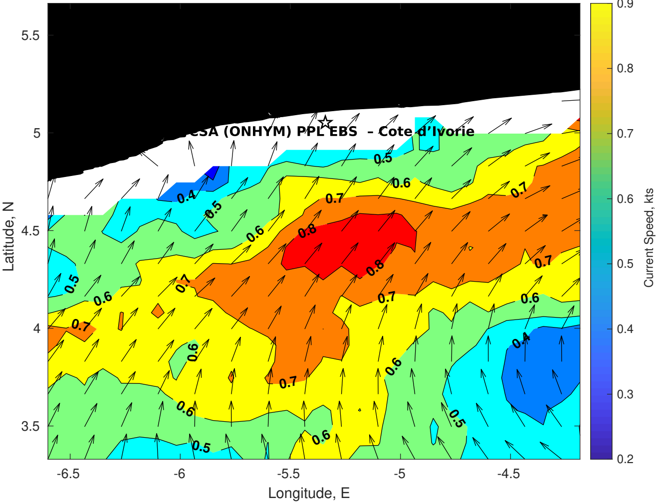
Surface Currents for CSA (ONHYM) PPL EBS - Cote d'Ivoire at 14-May-2025 00:00:00
