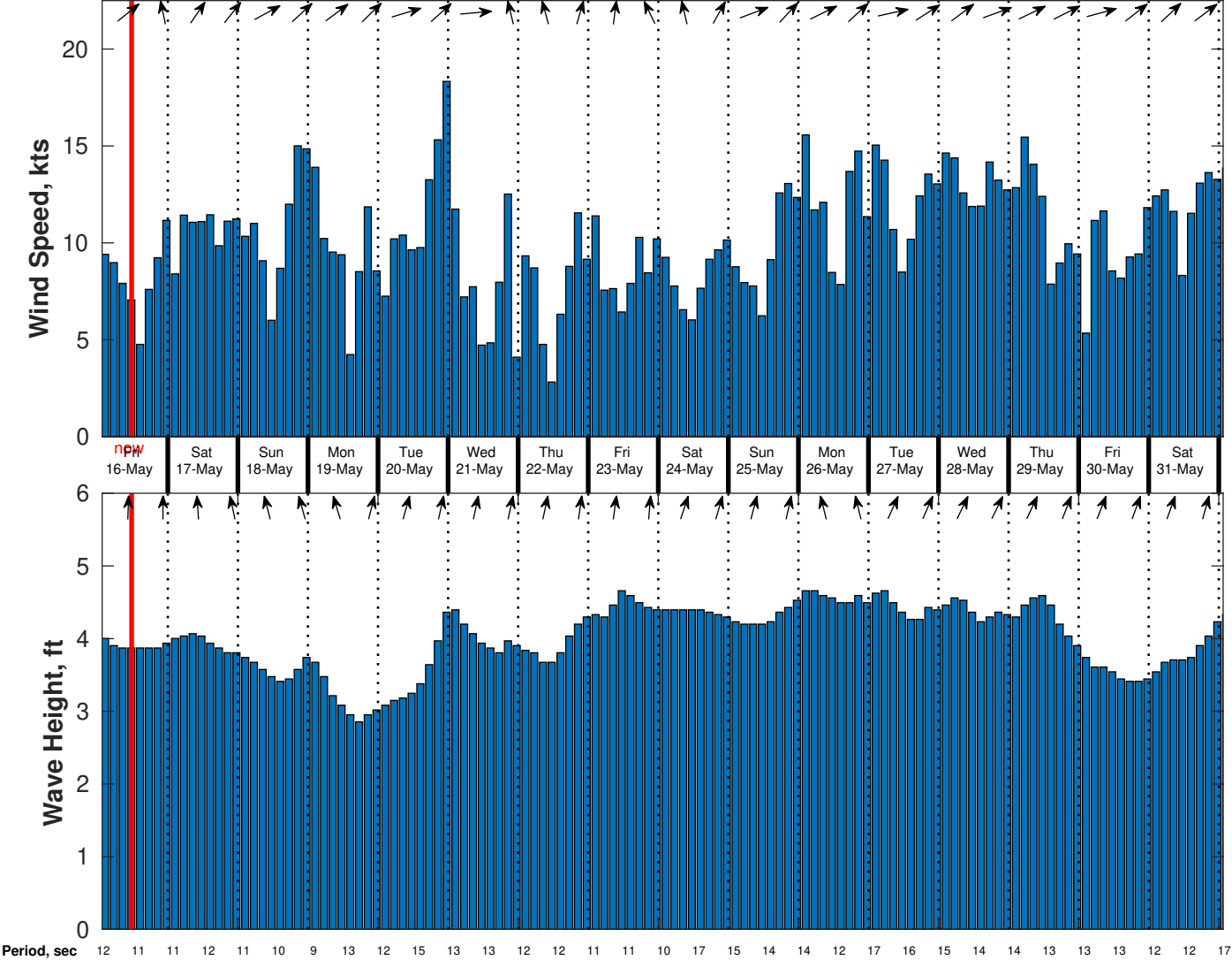
Wind & Wave Forecast for CSA (ONHYM) PPL EBS - Cote d'Ivoire from 15-May-2025 01:00:00 to 31-May-2025 01:00:00
