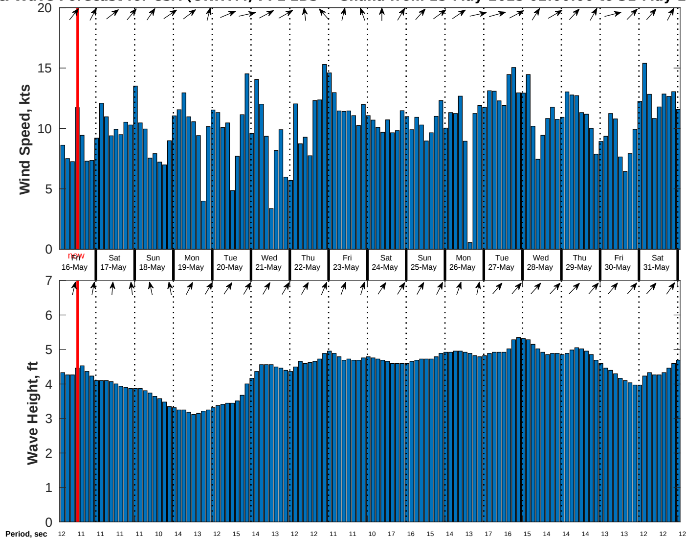
Wind & Wave Forecast for CSA (ONHYM) PPL EBS - Ghana from 15-May-2025 02:00:00 to 31-May-2025 02:00:00
