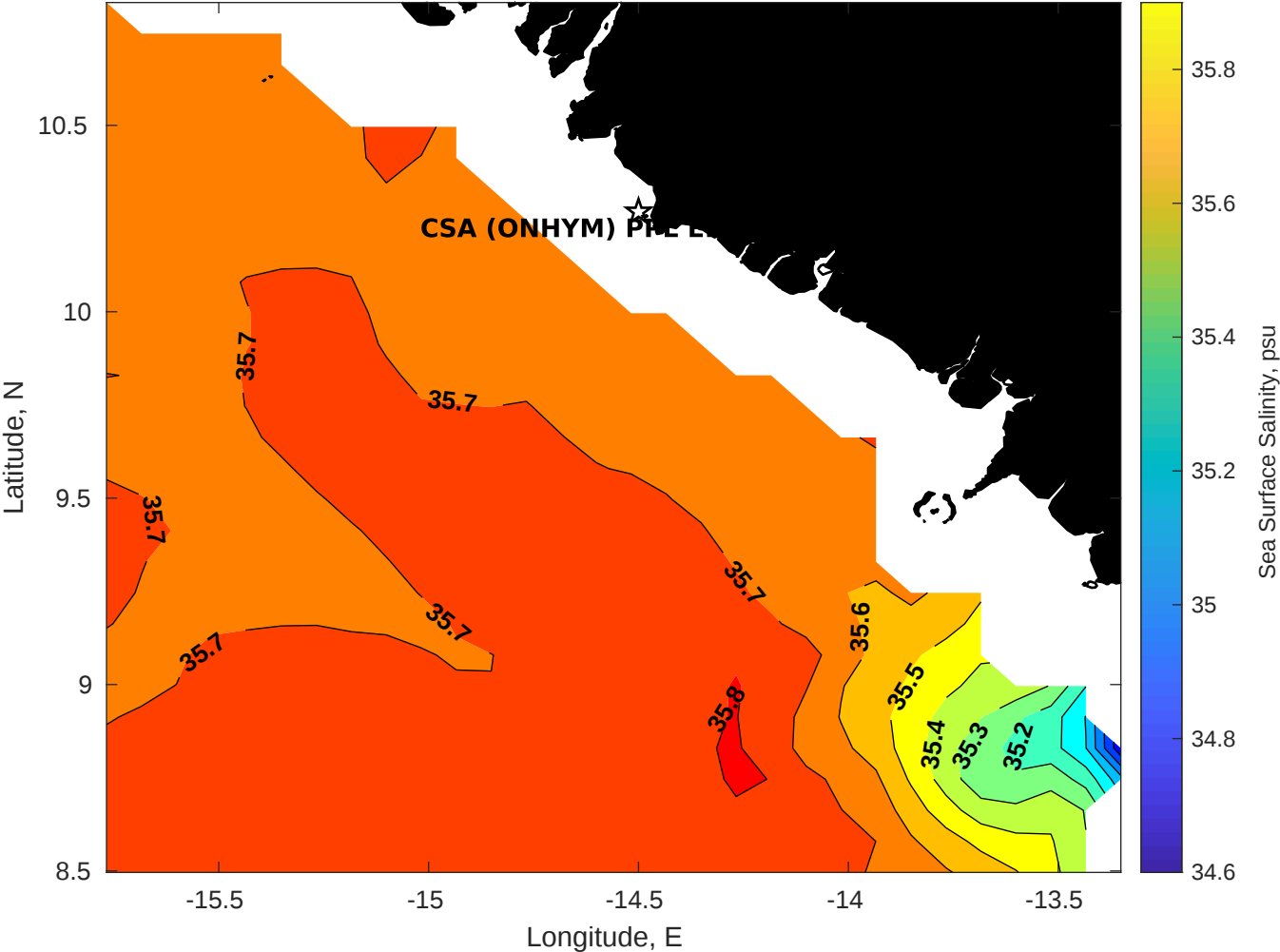
Surface Salinity for CSA (ONHYM) PPL EBS - Guinea at 14-May-2025 00:00:00
