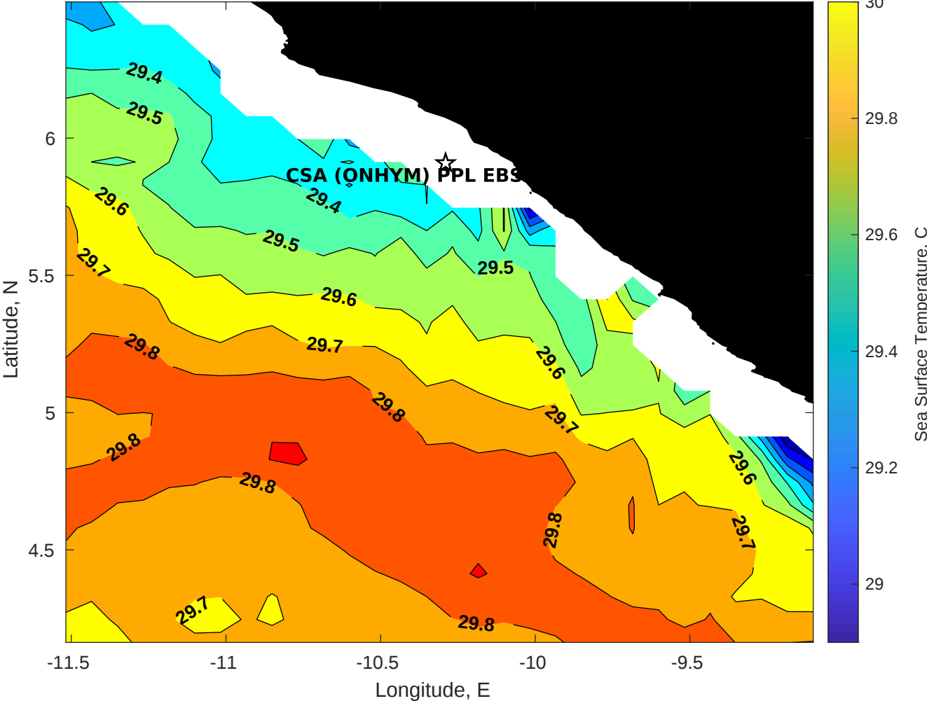
SST for CSA (ONHYM) PPL EBS - Liberia at 14-May-2025 00:00:00
