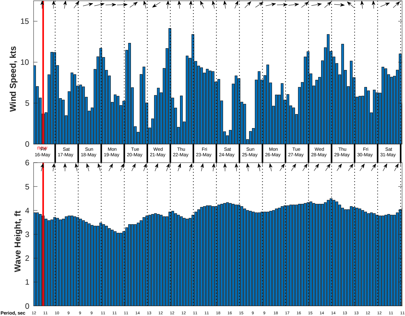
Wind & Wave Forecast for CSA (ONHYM) PPL EBS - Liberia from 15-May-2025 01:00:00 to 31-May-2025 01:00:00
