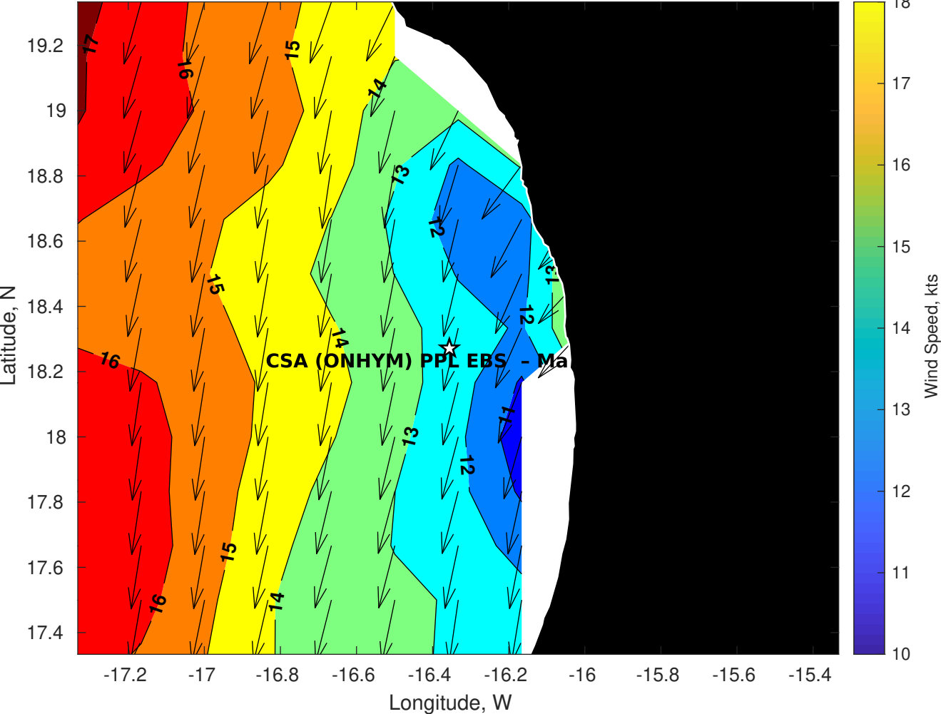
Winds (kts) for CSA (ONHYM) PPL EBS - Mauritania at 15-May-2025 09:00:00
