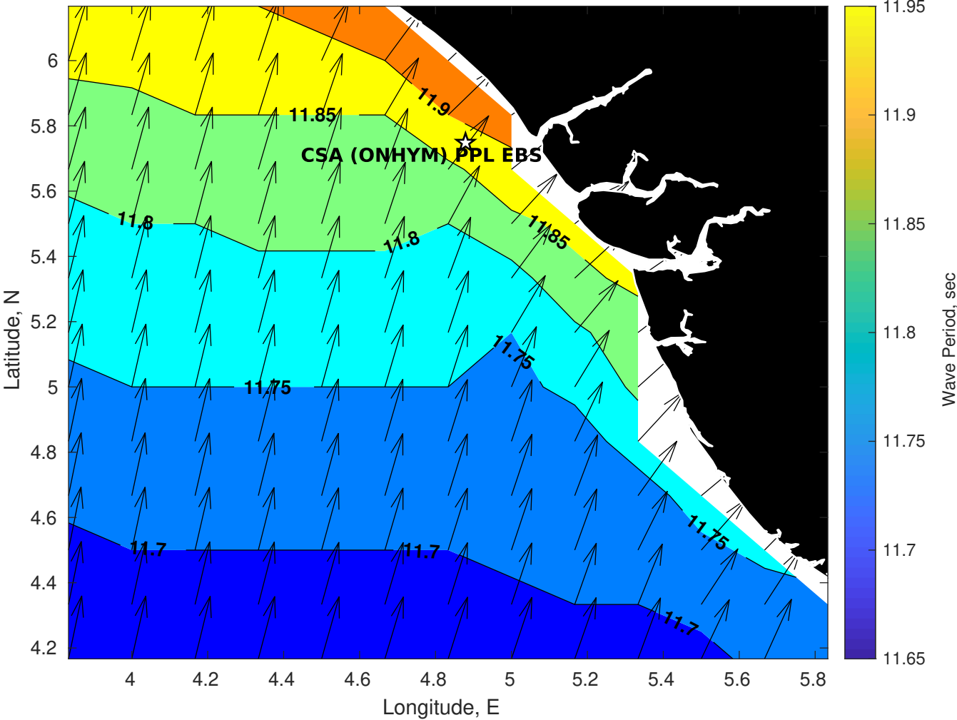
Wave Period (sec) for CSA (ONHYM) PPL EBS - Nigeria at 15-May-2025 09:00:00
