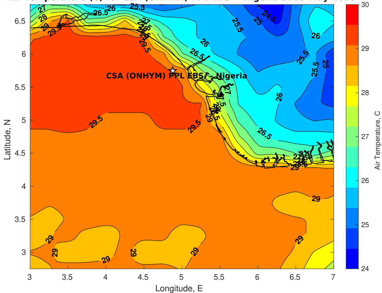
Air Temperature (C) for CSA (ONHYM) PPL EBS - Nigeria at 15-May-2025
