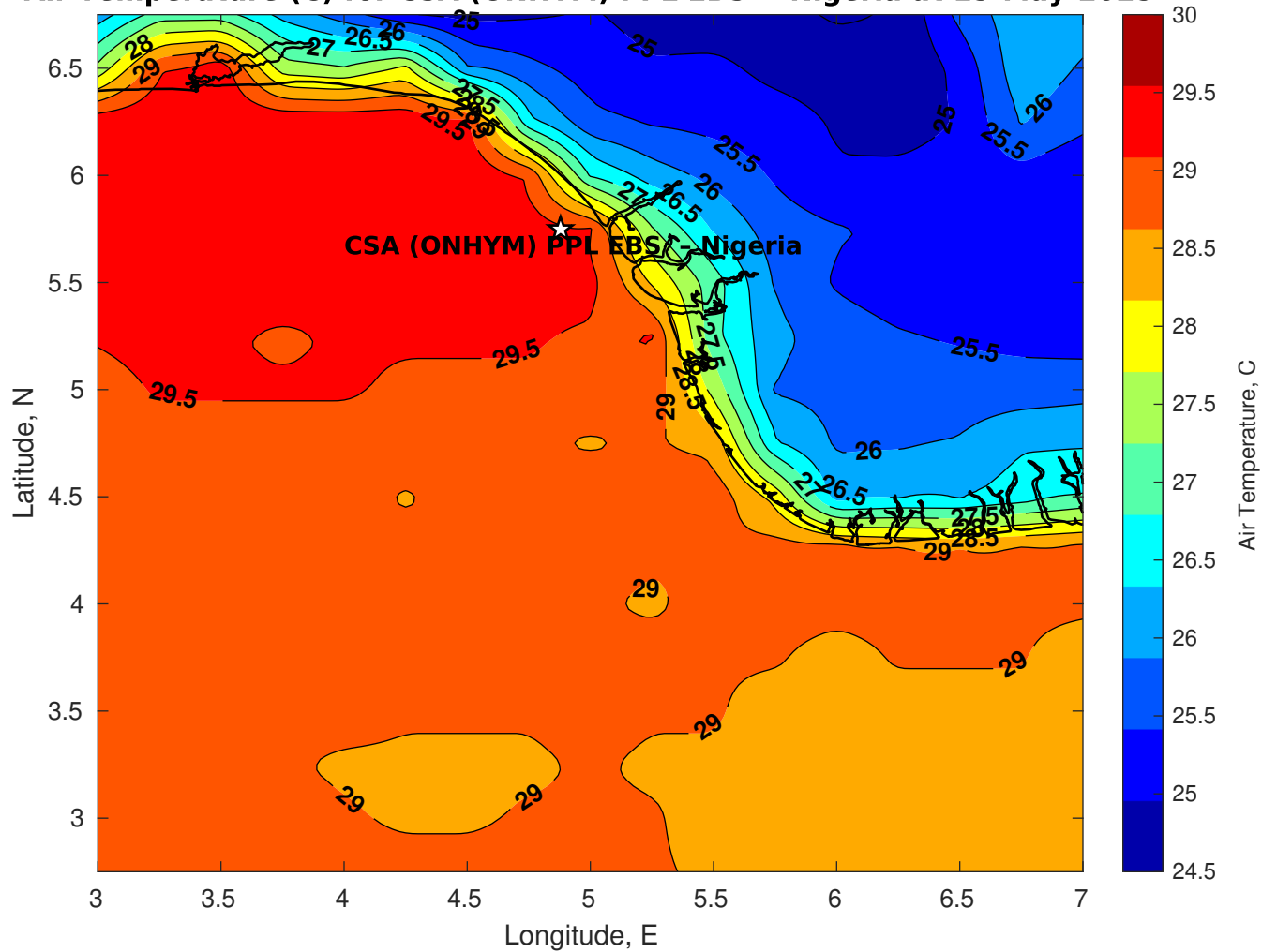
Air Temperature (C) for CSA (ONHYM) PPL EBS - Nigeria at 15-May-2025
