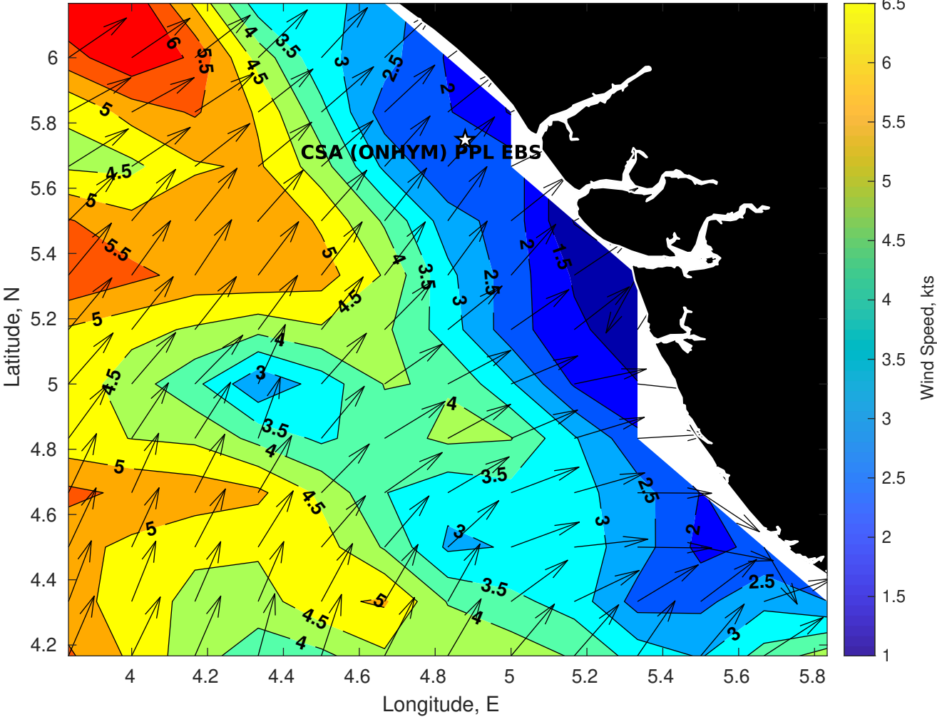
Winds (kts) for CSA (ONHYM) PPL EBS - Nigeria at 15-May-2025 09:00:00
