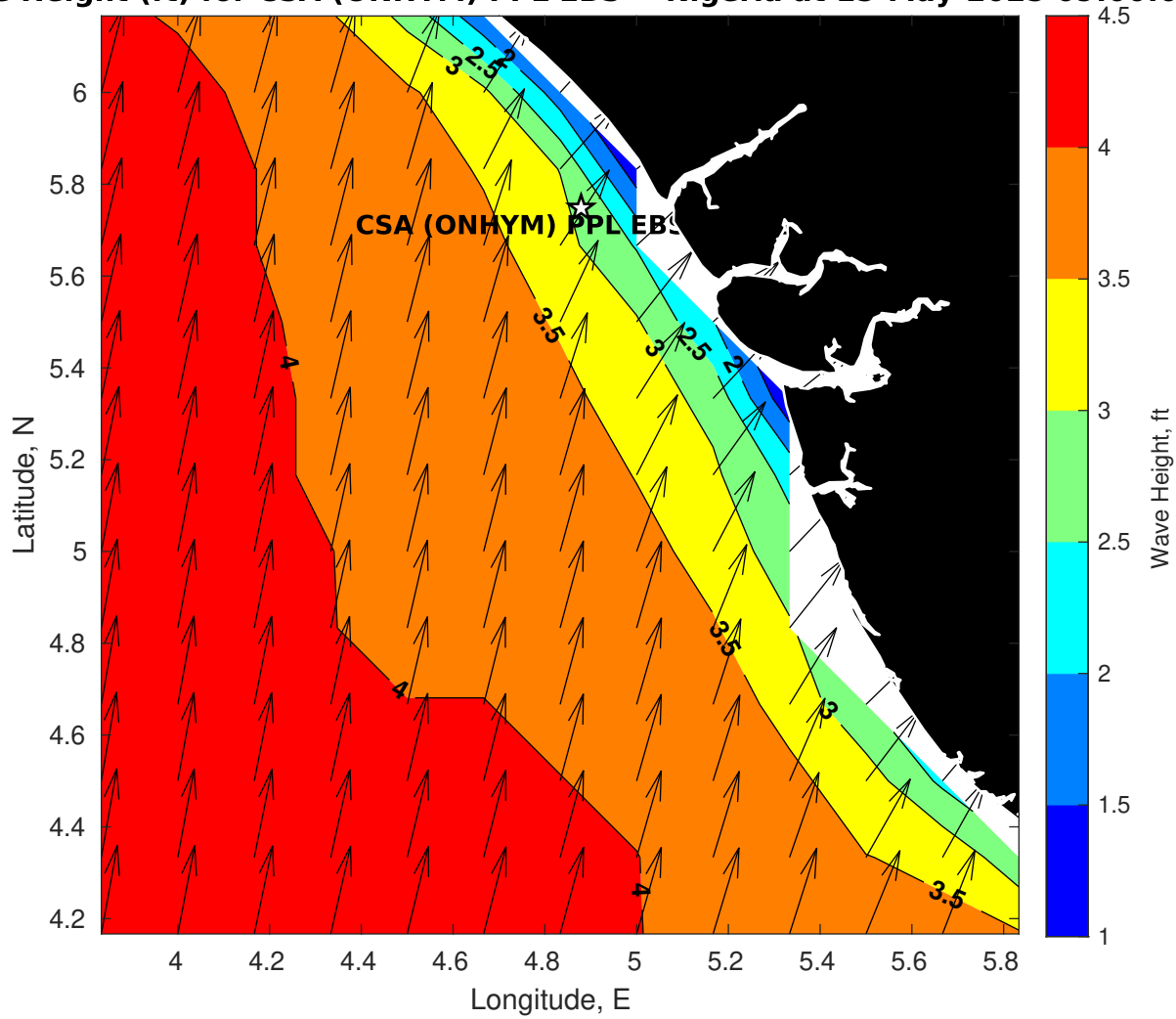
Wave Height (ft) for CSA (ONHYM) PPL EBS - Nigeria at 15-May-2025 09:00:00
