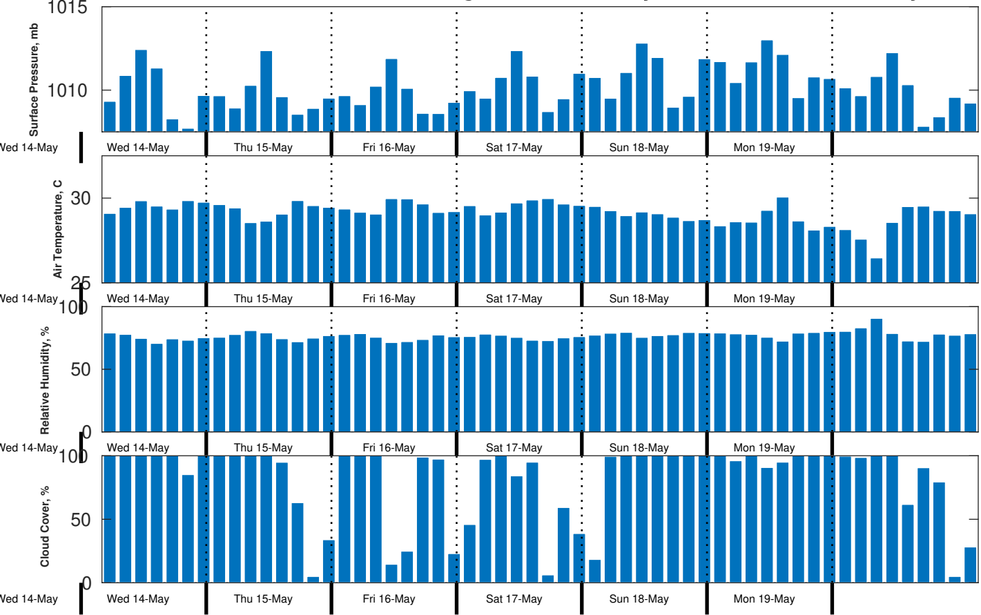
Met Forecast for CSA (ONHYM) PPL EBS - Nigeria from 15-May-2025 00:00:00 to 22-May-2025 00:00:00
