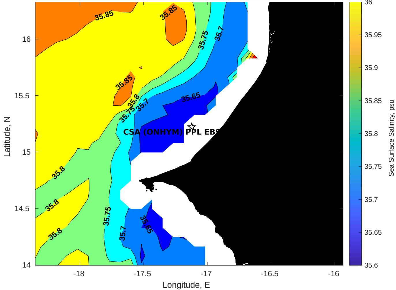
Surface Salinity for CSA (ONHYM) PPL EBS - Senegal at 14-May-2025 00:00:00
