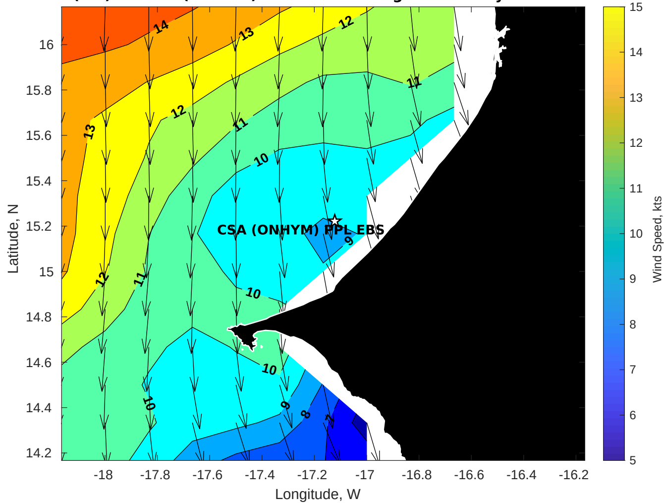
Winds (kts) for CSA (ONHYM) PPL EBS - Senegal at 15-May-2025 09:00:00
