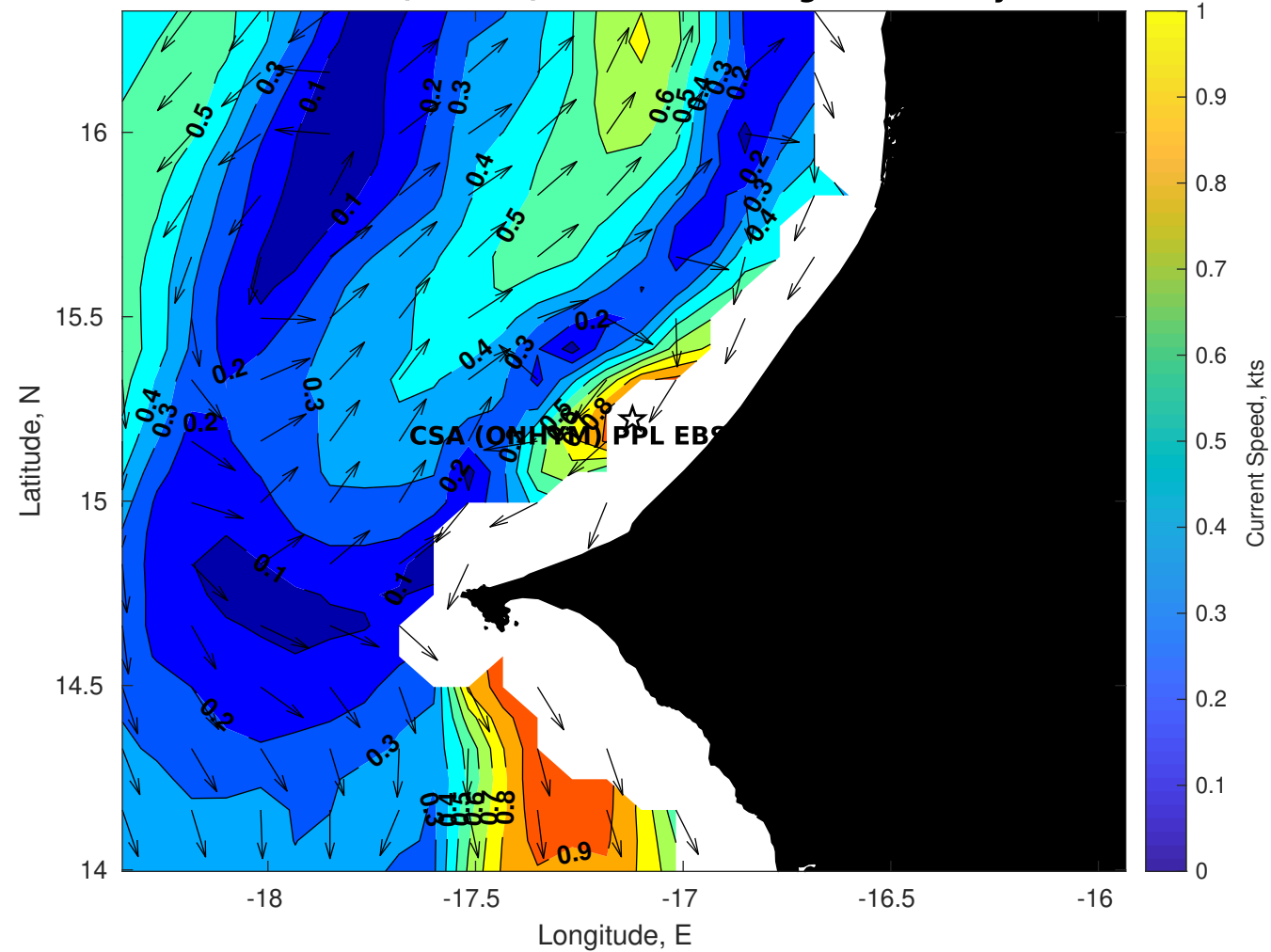
Surface Currents for CSA (ONHYM) PPL EBS - Senegal at 14-May-2025 00:00:00
