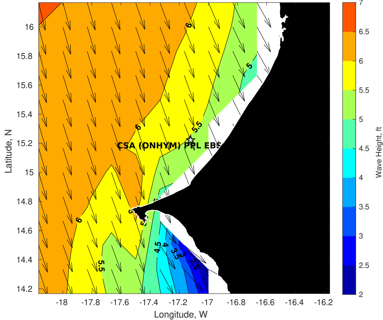
Wave Height (ft) for CSA (ONHYM) PPL EBS - Senegal at 15-May-2025 09:00:00
