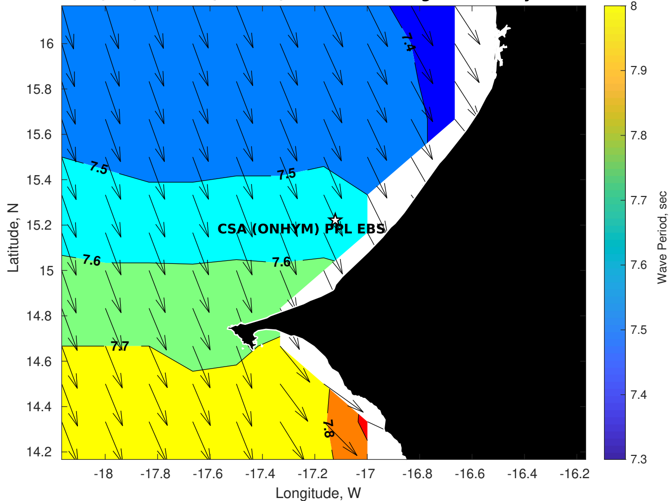
Wave Period (sec) for CSA (ONHYM) PPL EBS - Senegal at 15-May-2025 09:00:00
