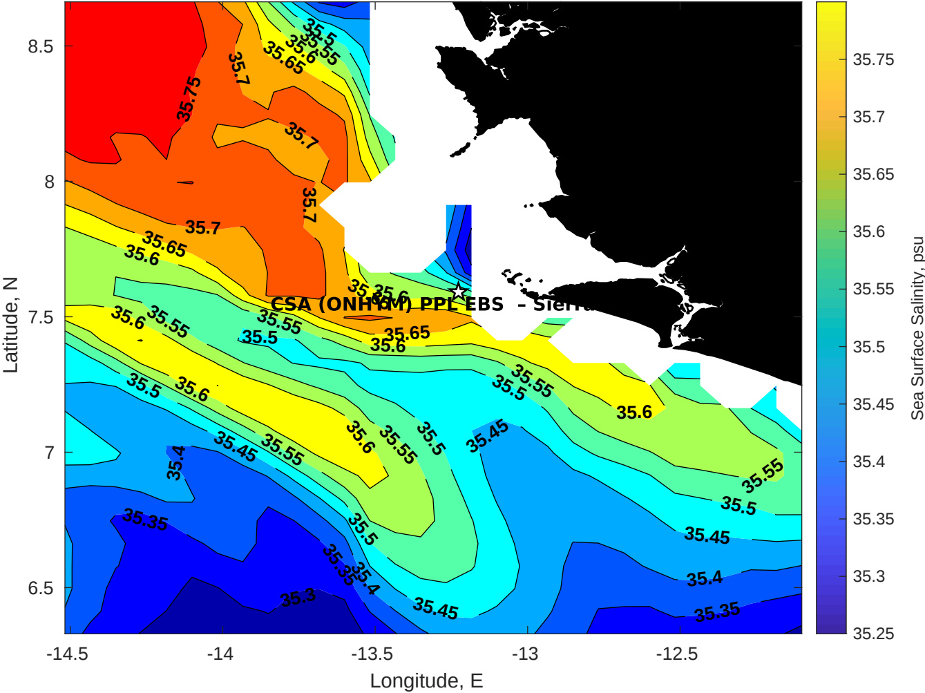
Surface Salinity for CSA (ONHYM) PPL EBS - Sierra Leone at 14-May-2025 00:00:00
