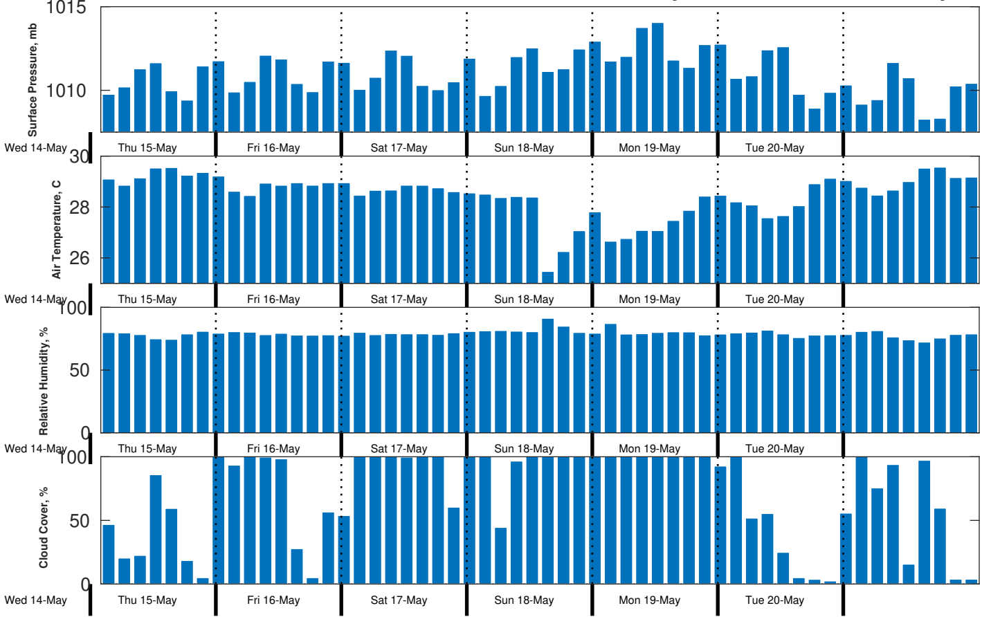
Met Forecast for CSA (ONHYM) PPL EBS - Sierra Leone from 15-May-2025 00:00:00 to 22-May-2025 00:00:00
