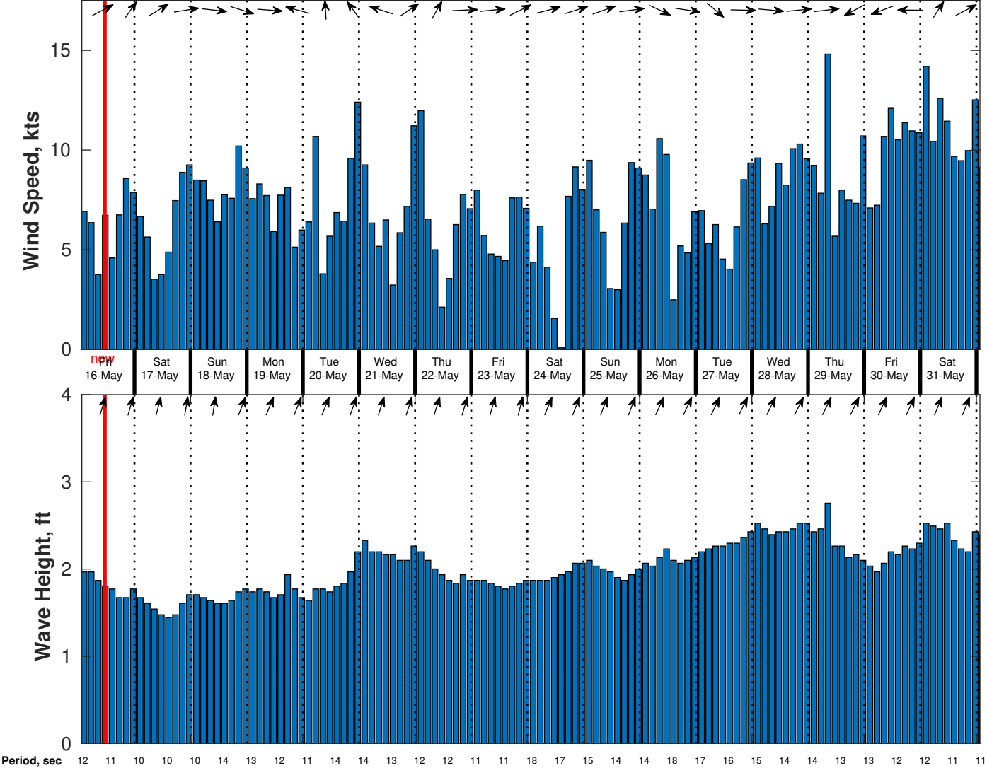
Wind & Wave Forecast for CSA (ONHYM) PPL EBS - Sierra Leone from 15-May-2025 01:00:00 to 31-May-2025 01:00:00
