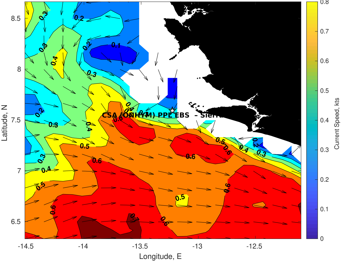
Surface Currents for CSA (ONHYM) PPL EBS - Sierra Leone at 14-May-2025 00:00:00
