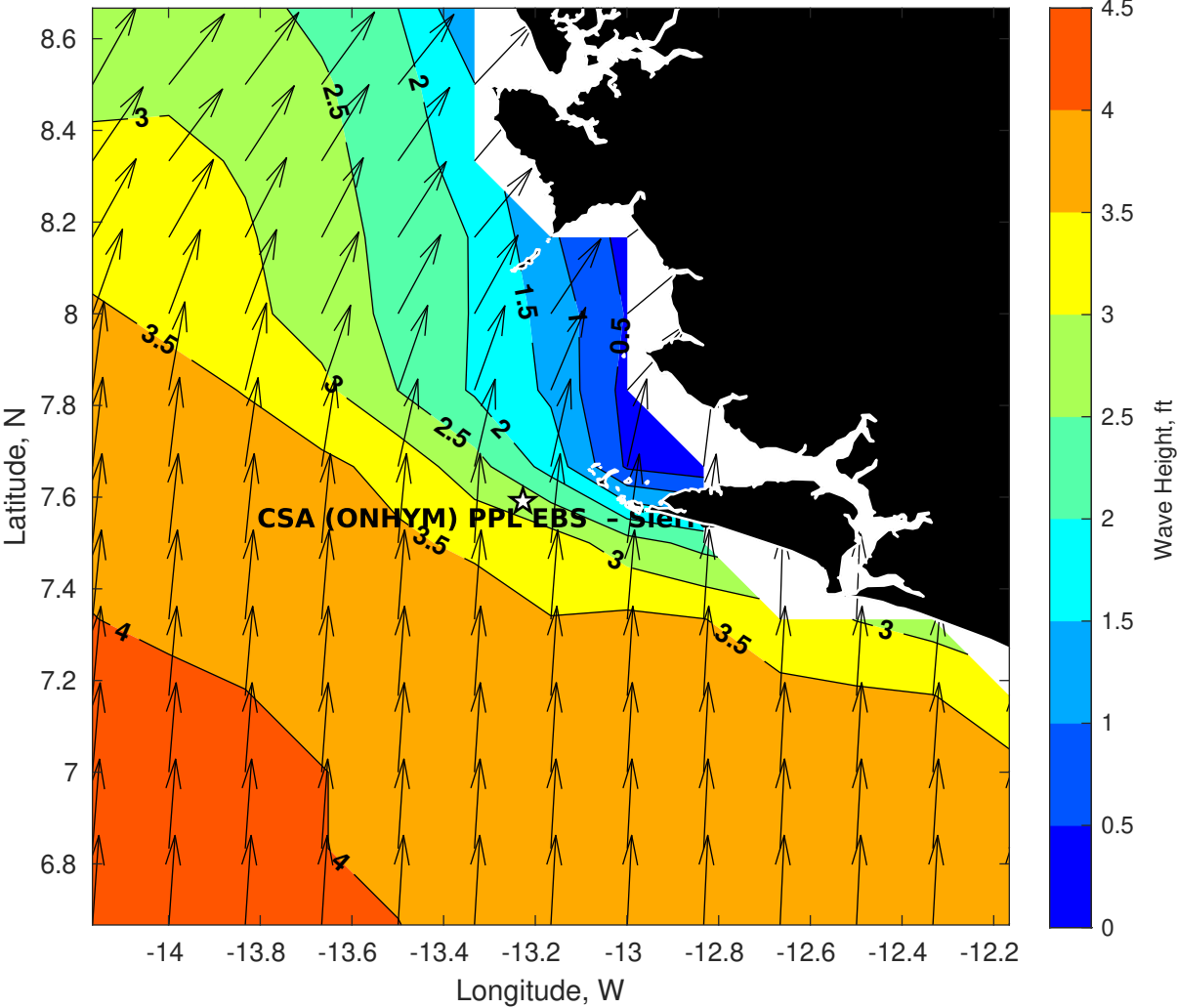
Wave Height (ft) for CSA (ONHYM) PPL EBS - Sierra Leone at 15-May-2025 09:00:00
