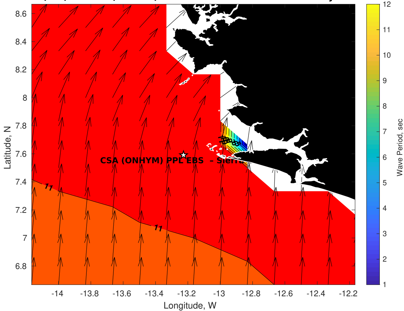
Wave Period (sec) for CSA (ONHYM) PPL EBS - Sierra Leone at 15-May-2025 09:00:00
