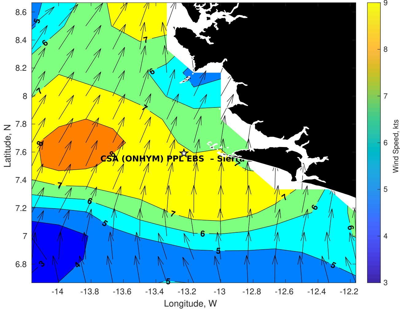
Winds (kts) for CSA (ONHYM) PPL EBS - Sierra Leone at 15-May-2025 09:00:00
