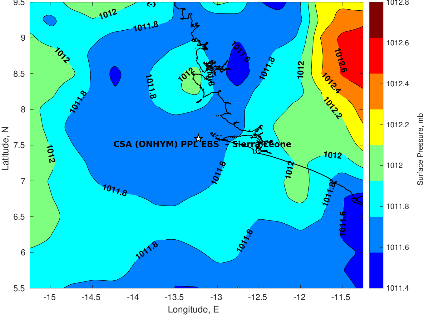
Surface Pressure (mb) for CSA (ONHYM) PPL EBS - Sierra Leone at 17-May-2025 00:00:00
