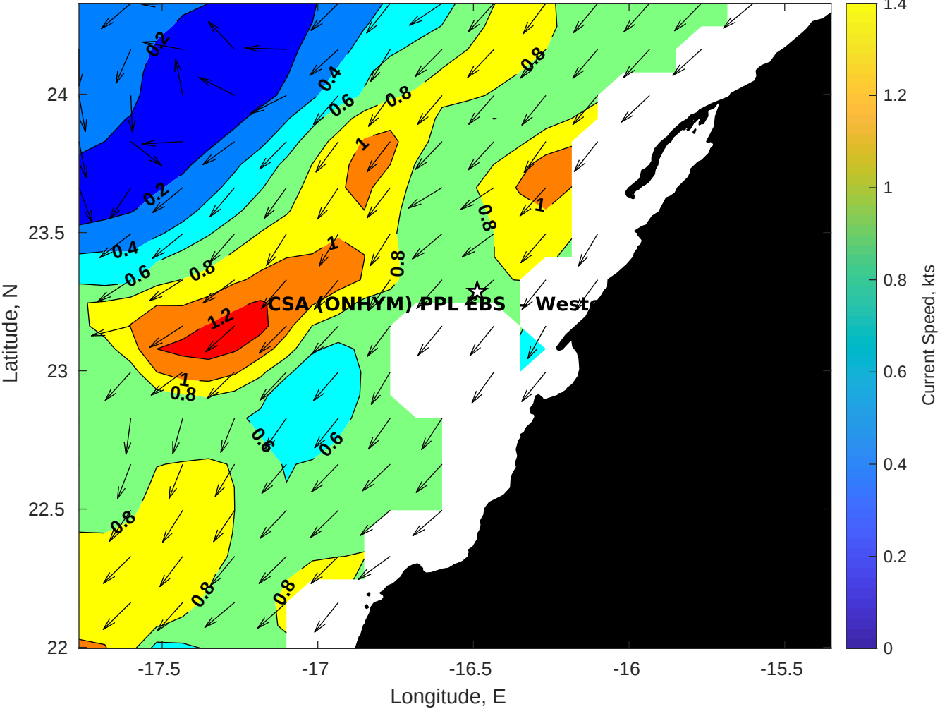
Surface Currents for CSA (ONHYM) PPL EBS - Western Sahara at 14-May-2025 00:00:00
