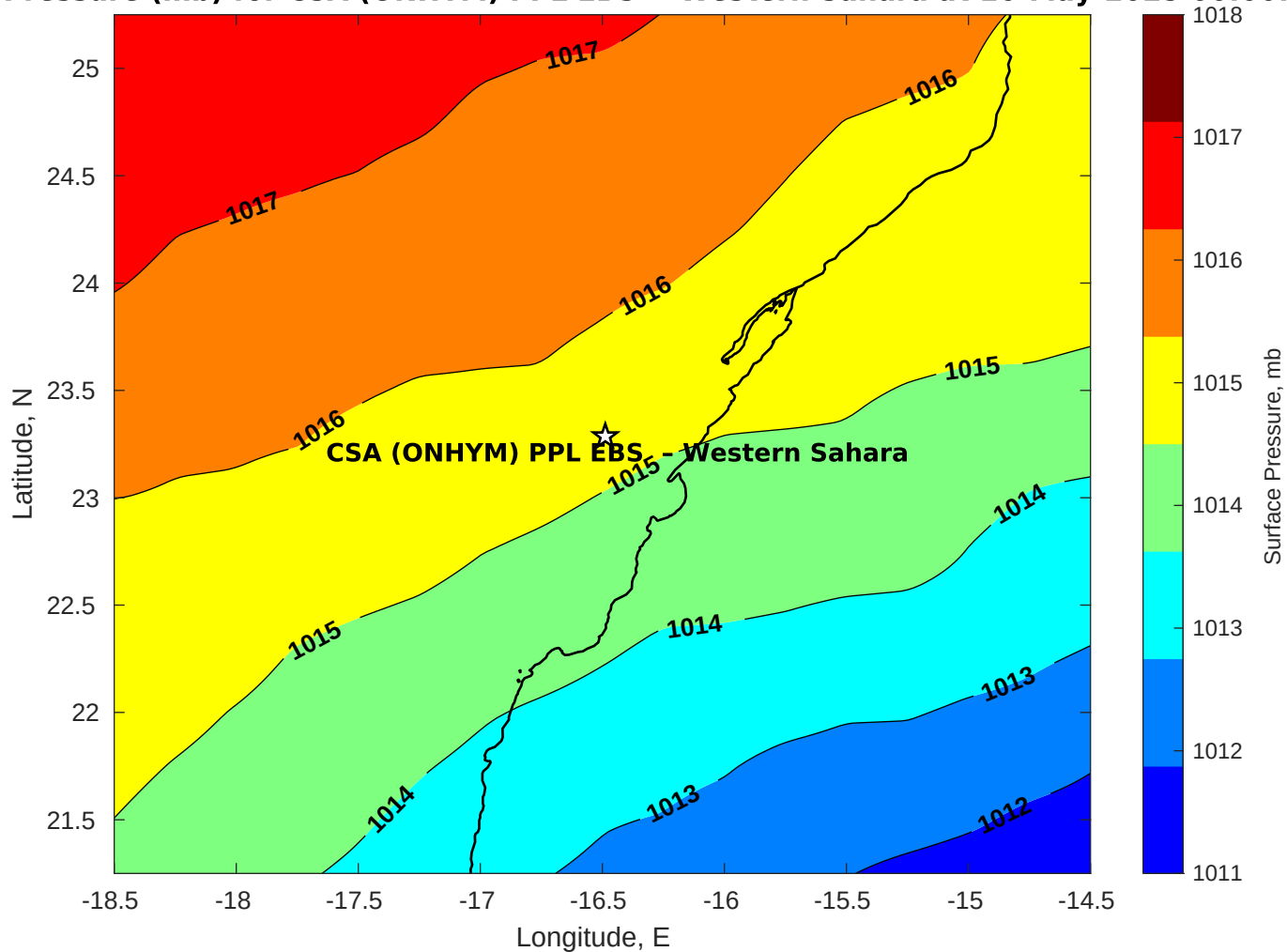
Surface Pressure (mb) for CSA (ONHYM) PPL EBS - Western Sahara at 16-May-2025 00:00:00
