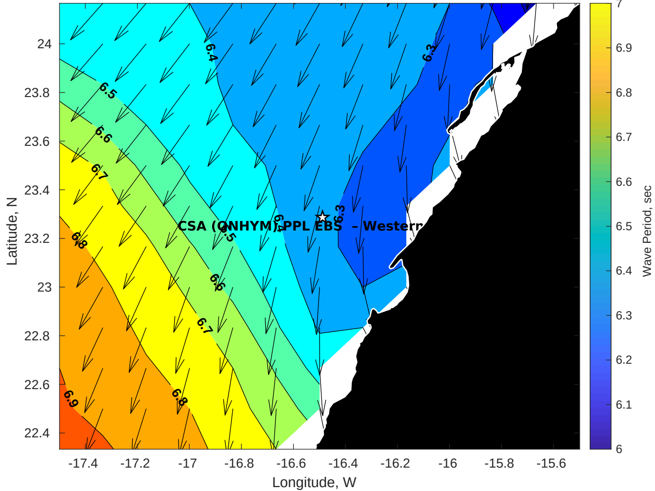
Wave Period (sec) for CSA (ONHYM) PPL EBS - Western Sahara at 15-May-2025 09:00:00
