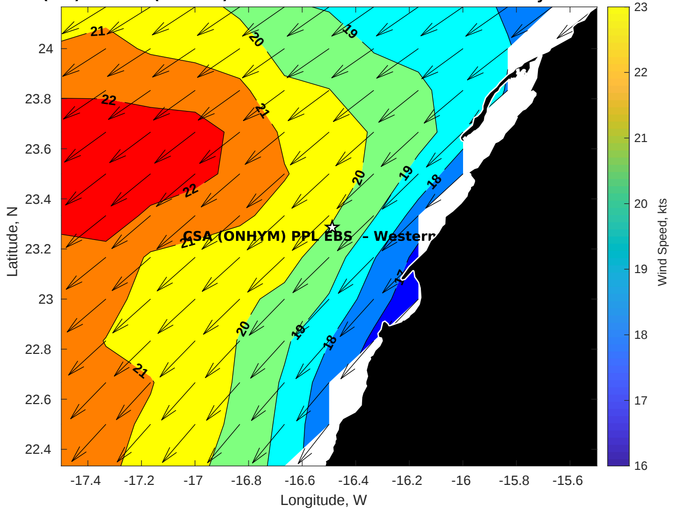
Winds (kts) for CSA (ONHYM) PPL EBS - Western Sahara at 15-May-2025 09:00:00
