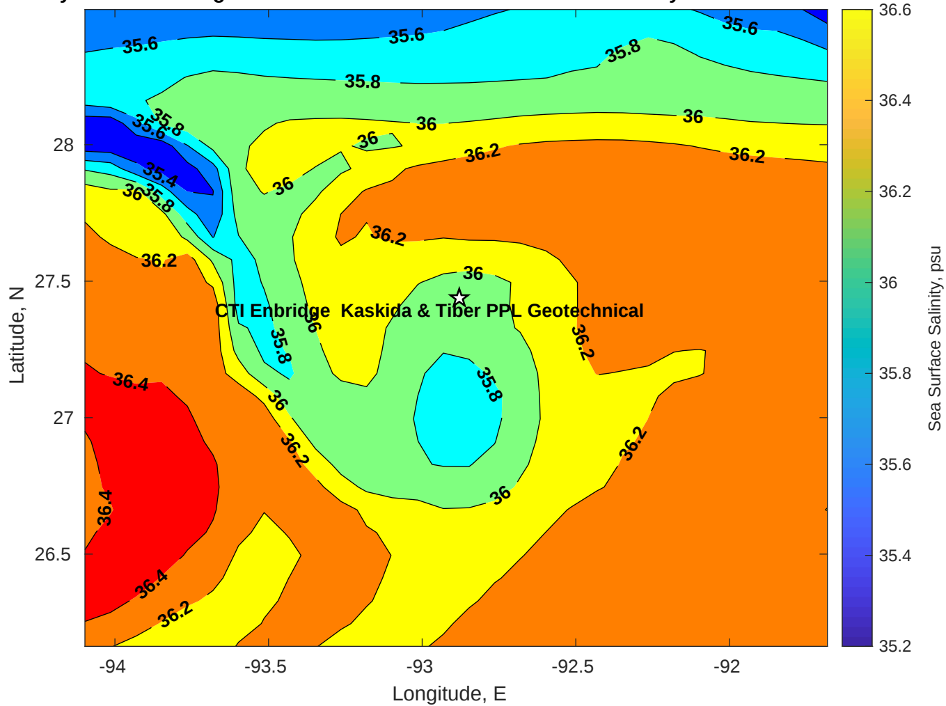
Surface Salinity for CTI Enbridge Kaskida & Tiber PPL Geotechnical at 14-May-2025 00:00:00
