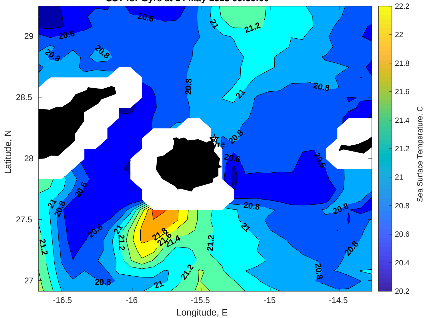
SST for Gyre at 14-May-2025 00:00:00
