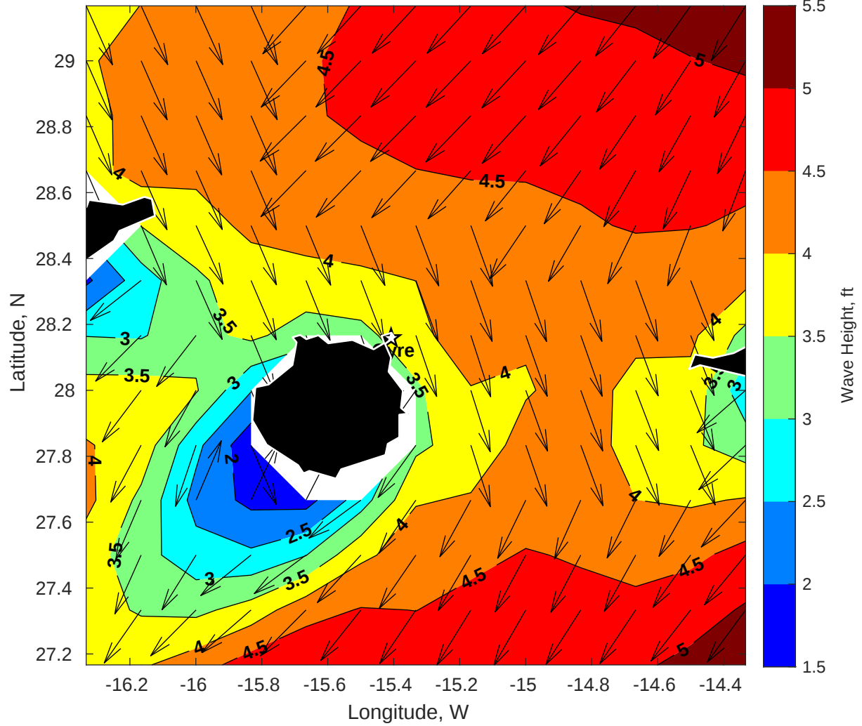
Wave Height (ft) for Gyre at 15-May-2025 09:00:00
