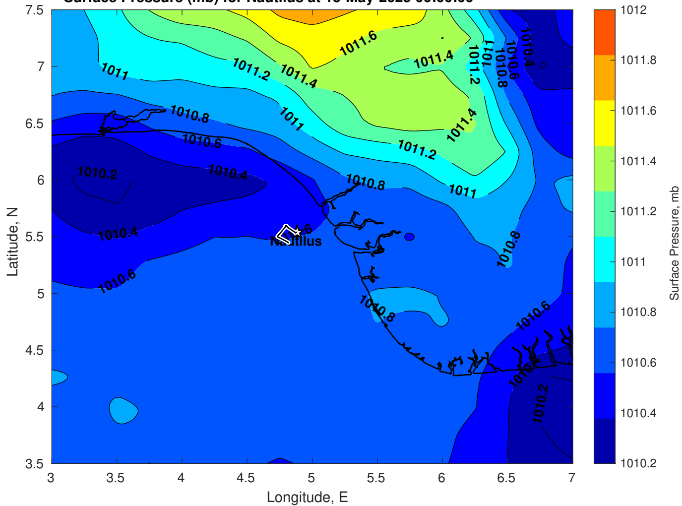
Surface Pressure (mb) for Nautilus at 15-May-2025 00:00:00
