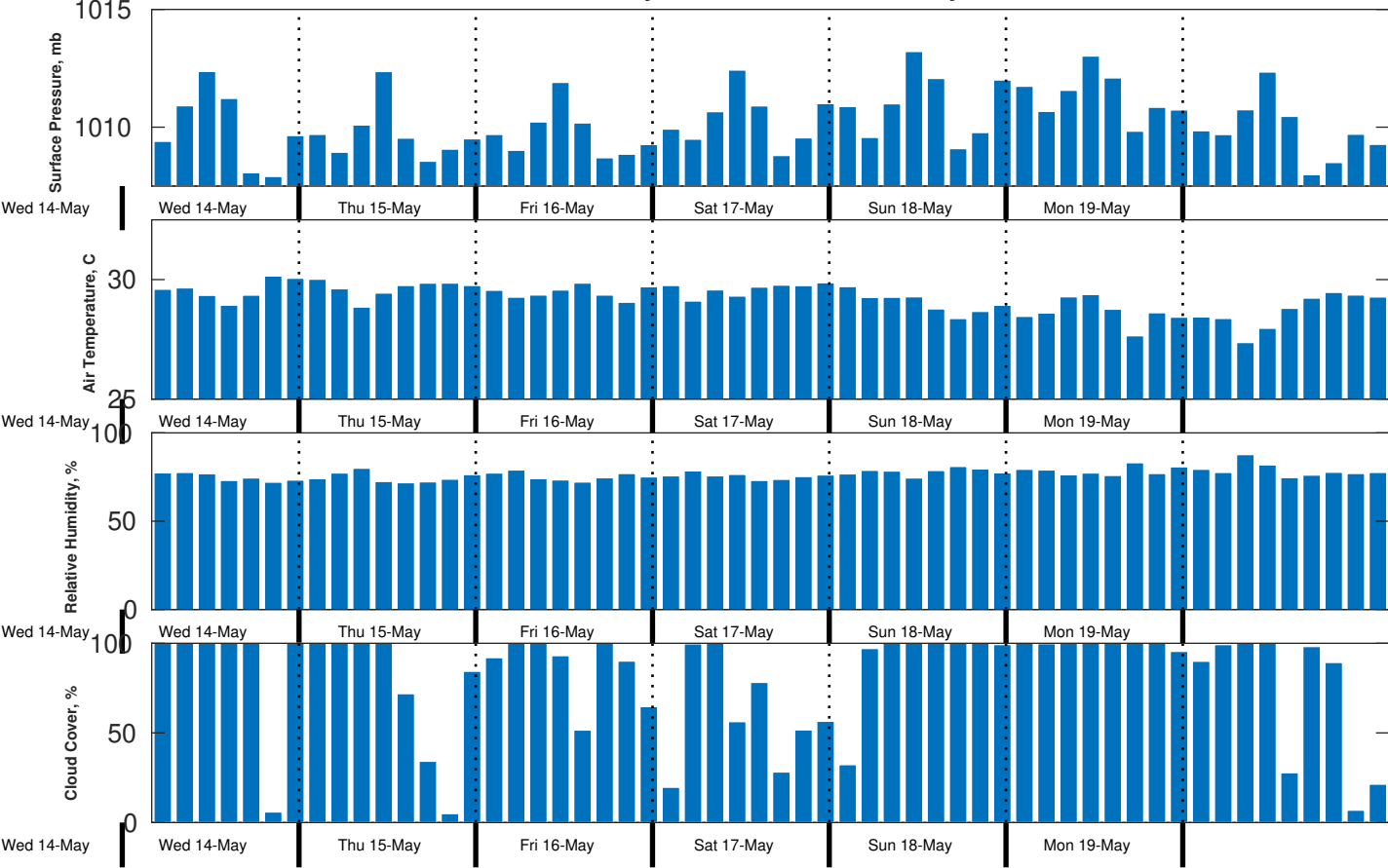
Met Forecast for Nautilus from 15-May-2025 00:00:00 to 22-May-2025 00:00:00
