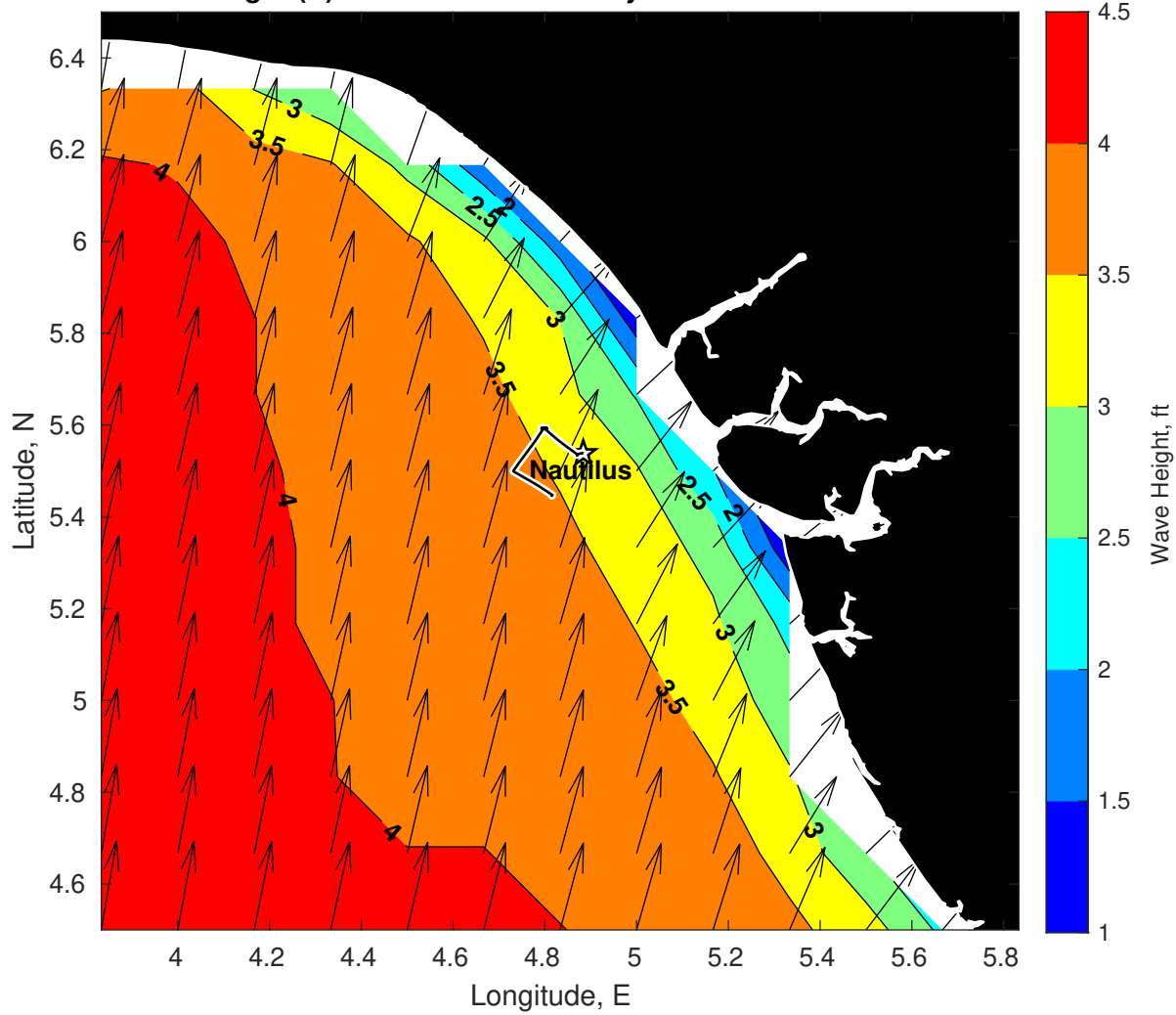
Wave Height (ft) for Nautilus at 15-May-2025 09:00:00
