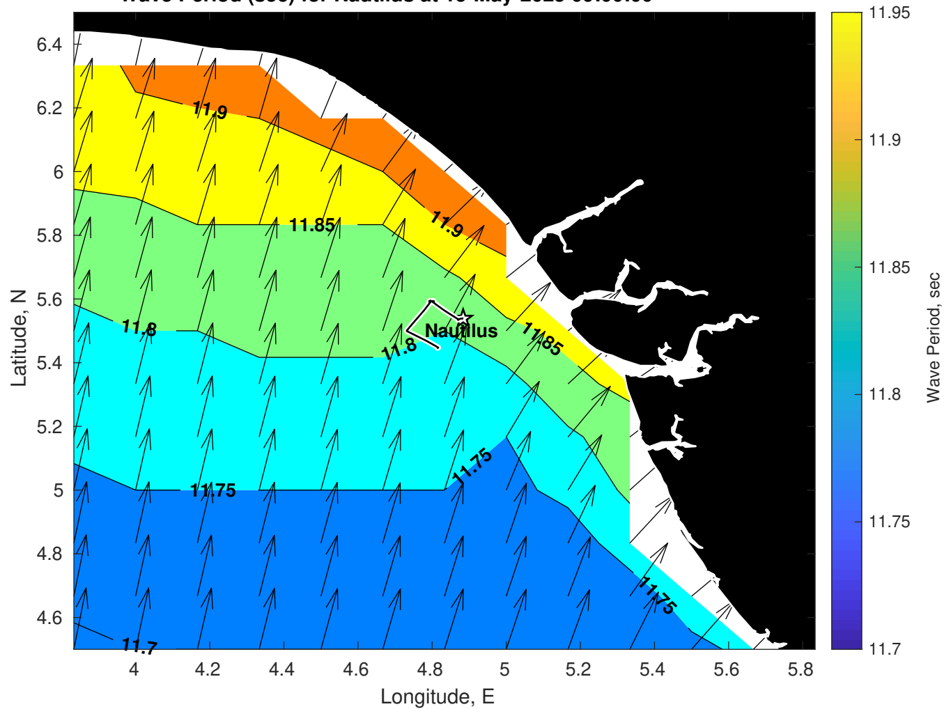
Wave Period (sec) for Nautilus at 15-May-2025 09:00:00
