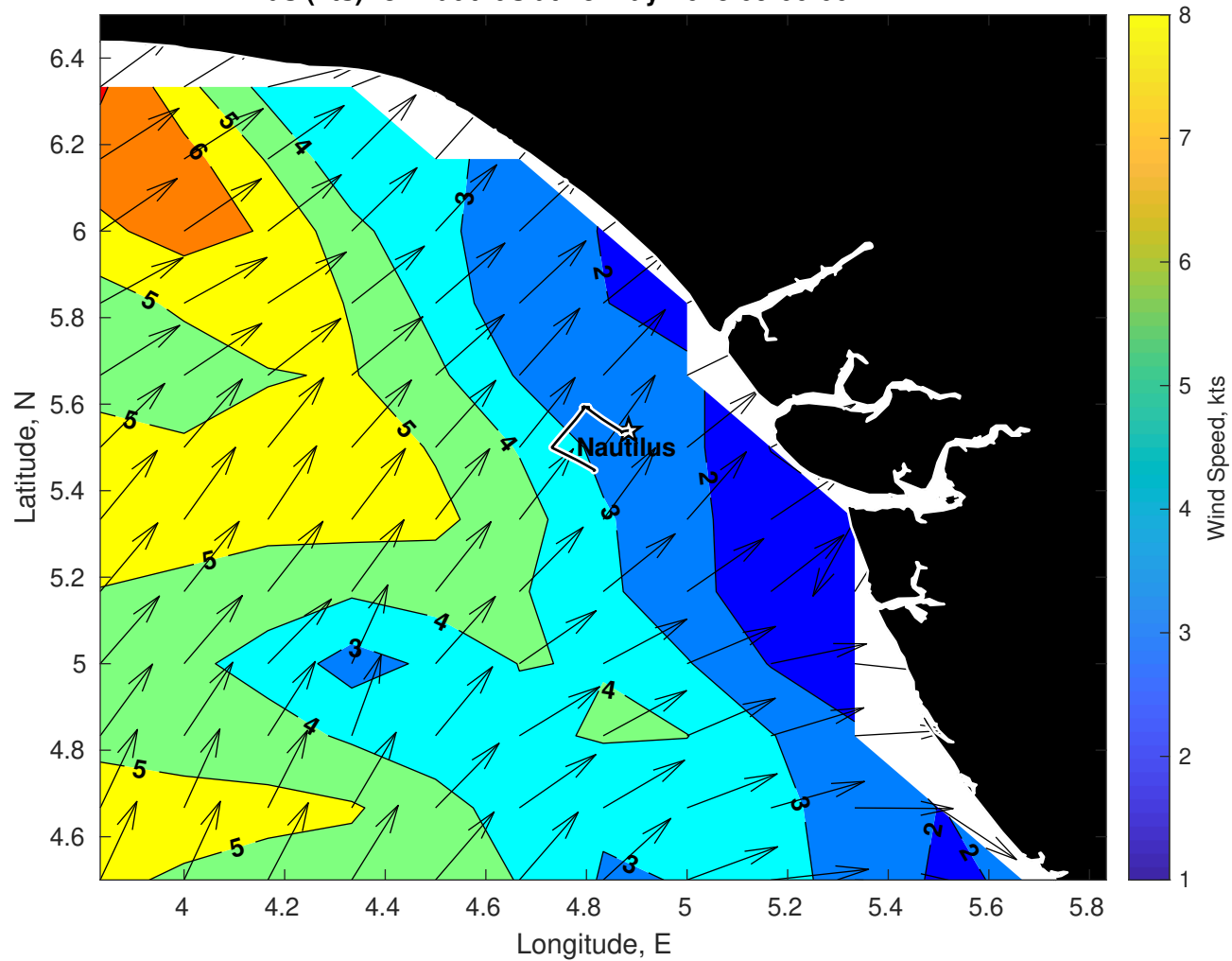
Winds (kts) for Nautilus at 15-May-2025 09:00:00
