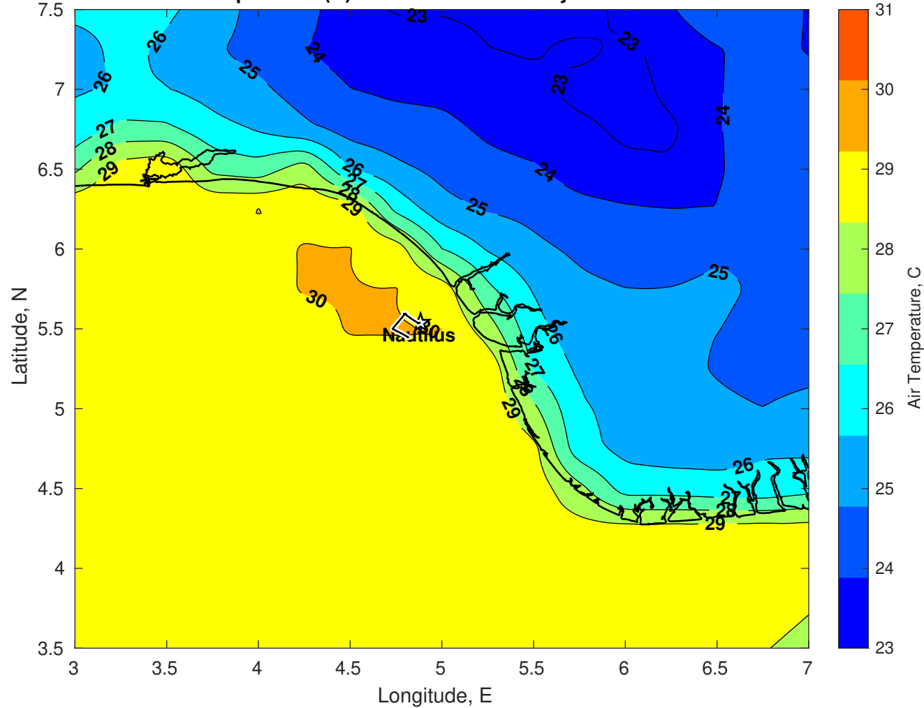
Air Temperature (C) for Nautilus at 15-May-2025
