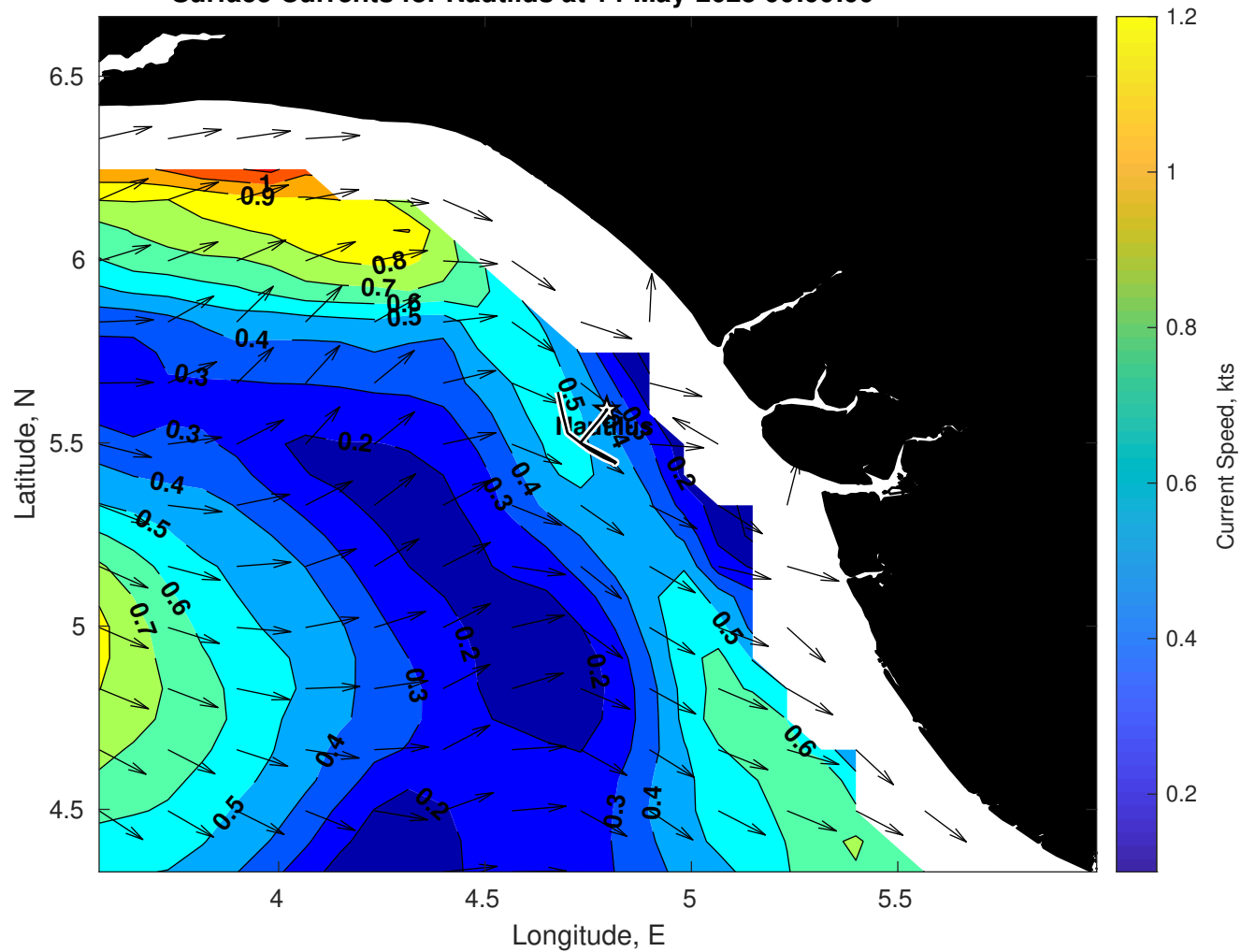
Surface Currents for Nautilus at 14-May-2025 00:00:00
