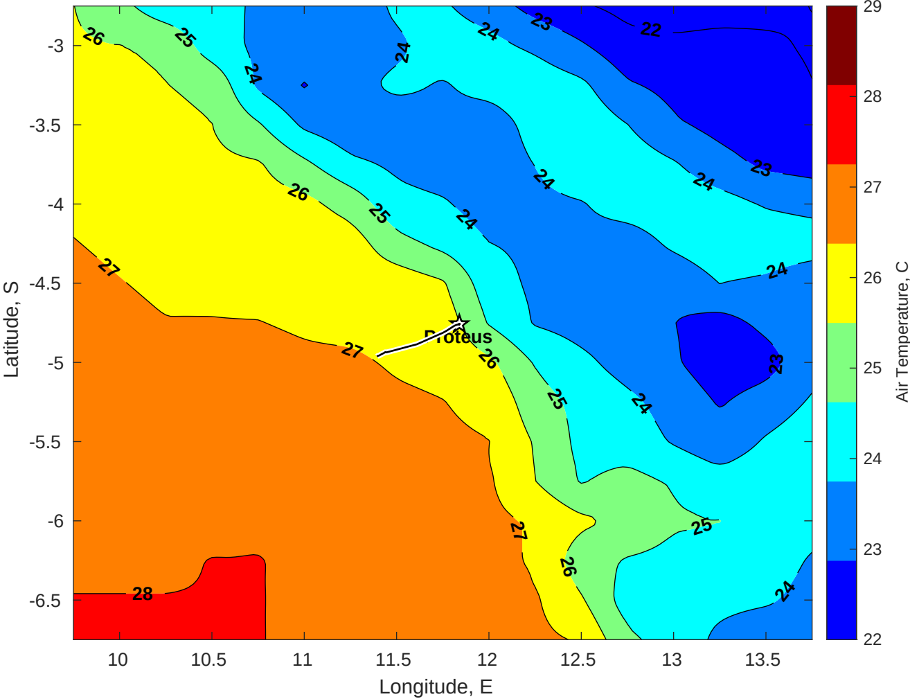
Air Temperature (C) for Proteus at 15-May-2025
