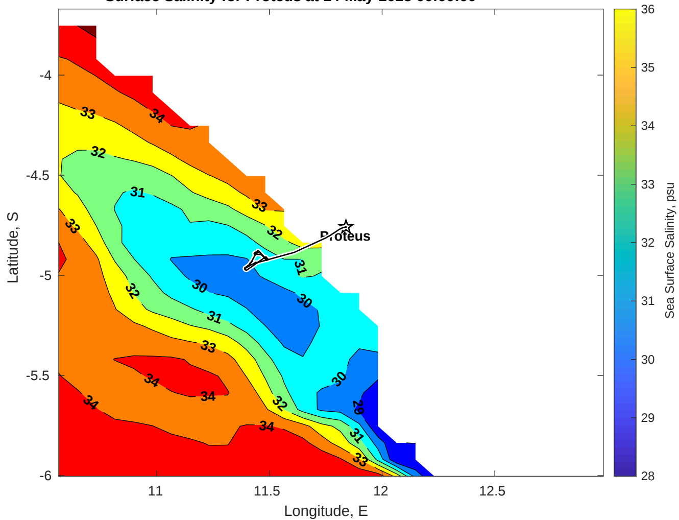
Surface Salinity for Proteus at 14-May-2025 00:00:00
