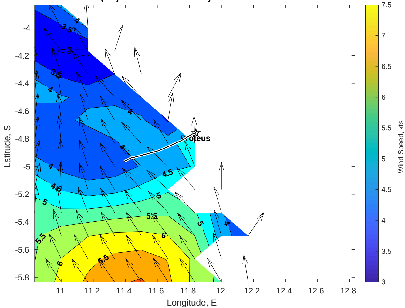
Winds (kts) for Proteus at 15-May-2025 09:00:00
