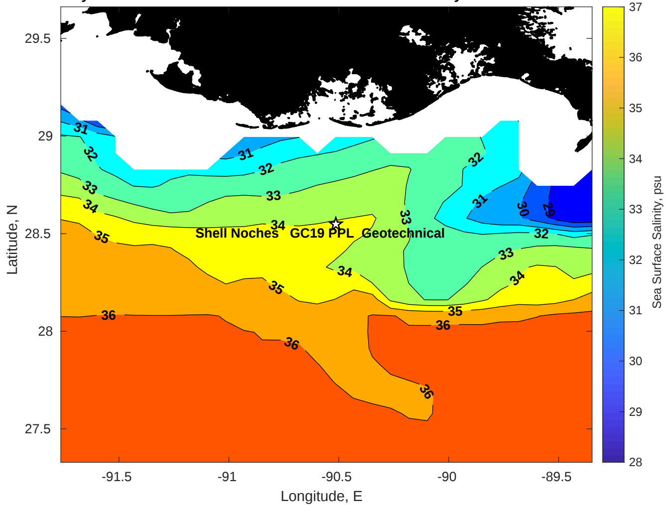
Surface Salinity for Shell Noches GC19 PPL Geotechnical at 14-May-2025 00:00:00
