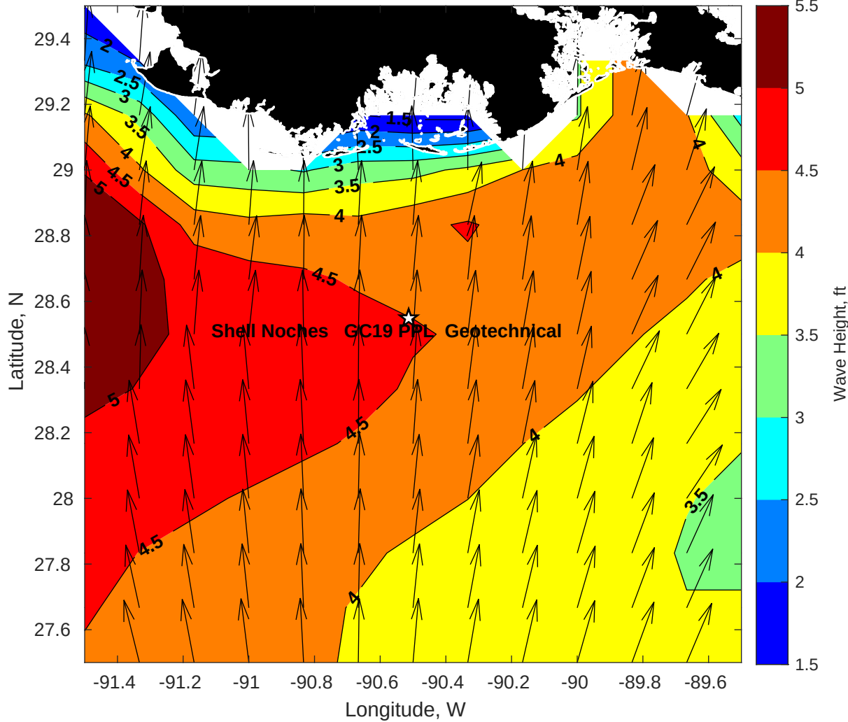
Wave Height (ft) for Shell Noches GC19 PPL Geotechnical at 15-May-2025 09:00:00
