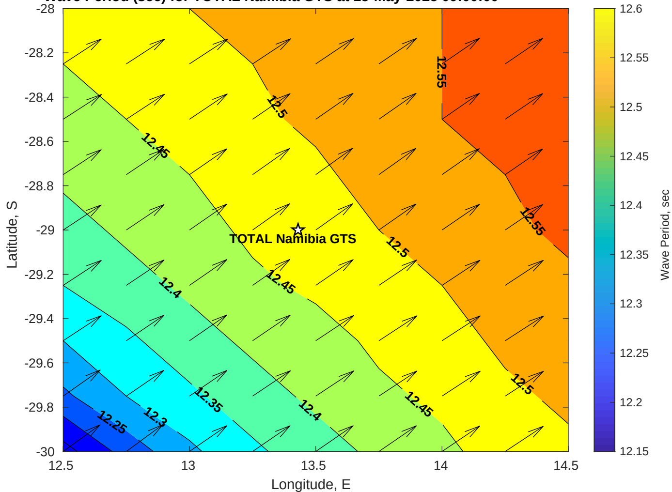
Wave Period (sec) for TOTAL Namibia GTS at 15-May-2025 09:00:00
