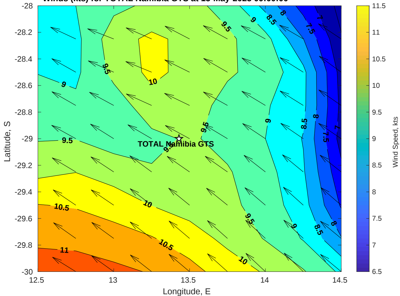
Winds (kts) for TOTAL Namibia GTS at 15-May-2025 09:00:00
