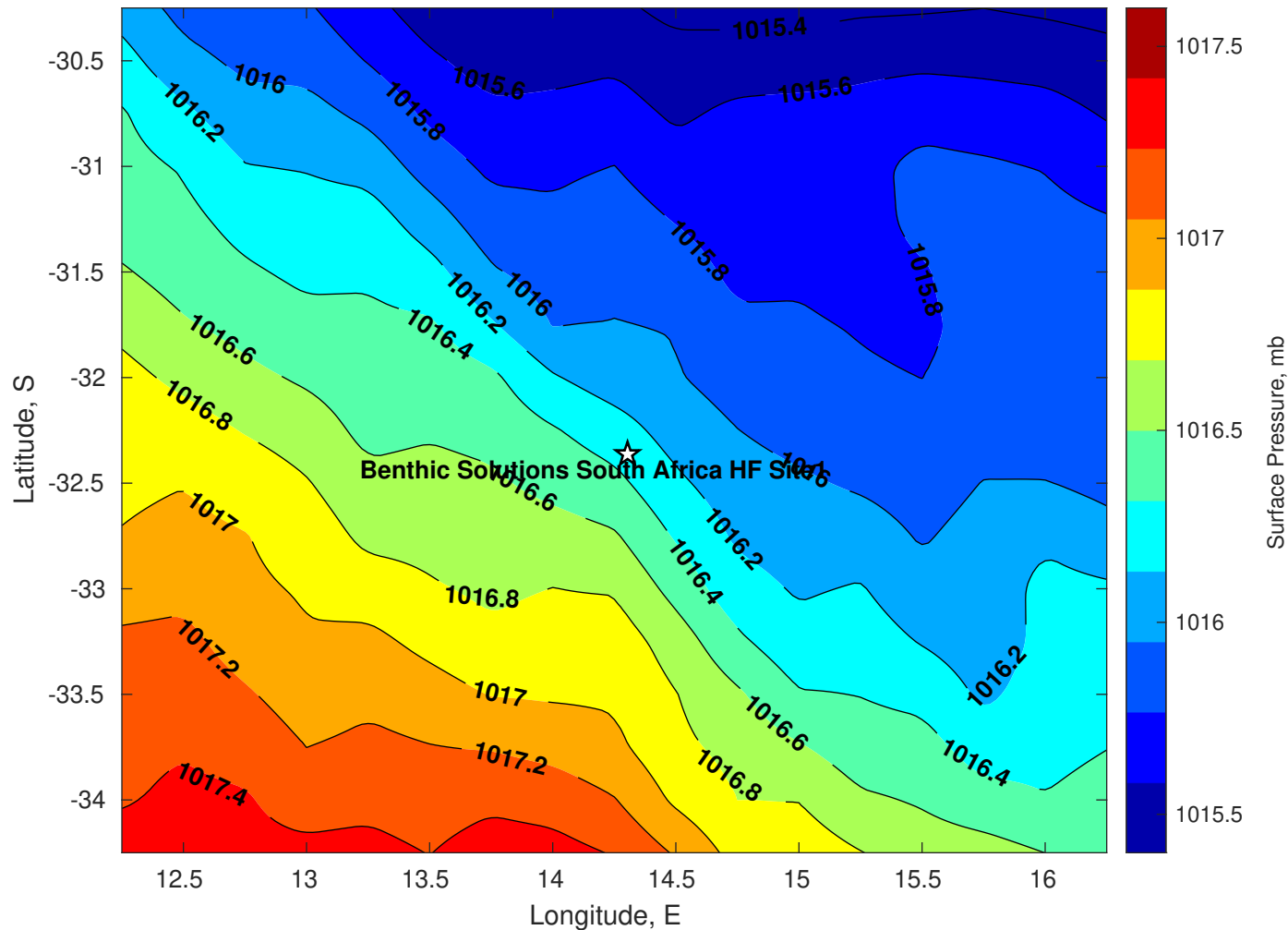
Surface Pressure (mb) for Benthic Solutions South Africa HF Site1 at 16-May-2025 00:00:00
