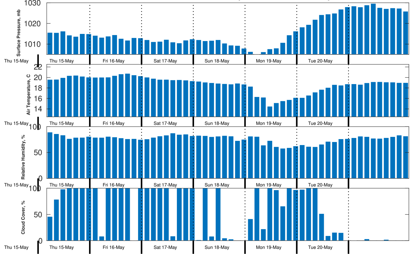
Met Forecast for Benthic Solutions South Africa HF Site1 from 16-May-2025 00:00:00 to 23-May-2025 00:00:00
