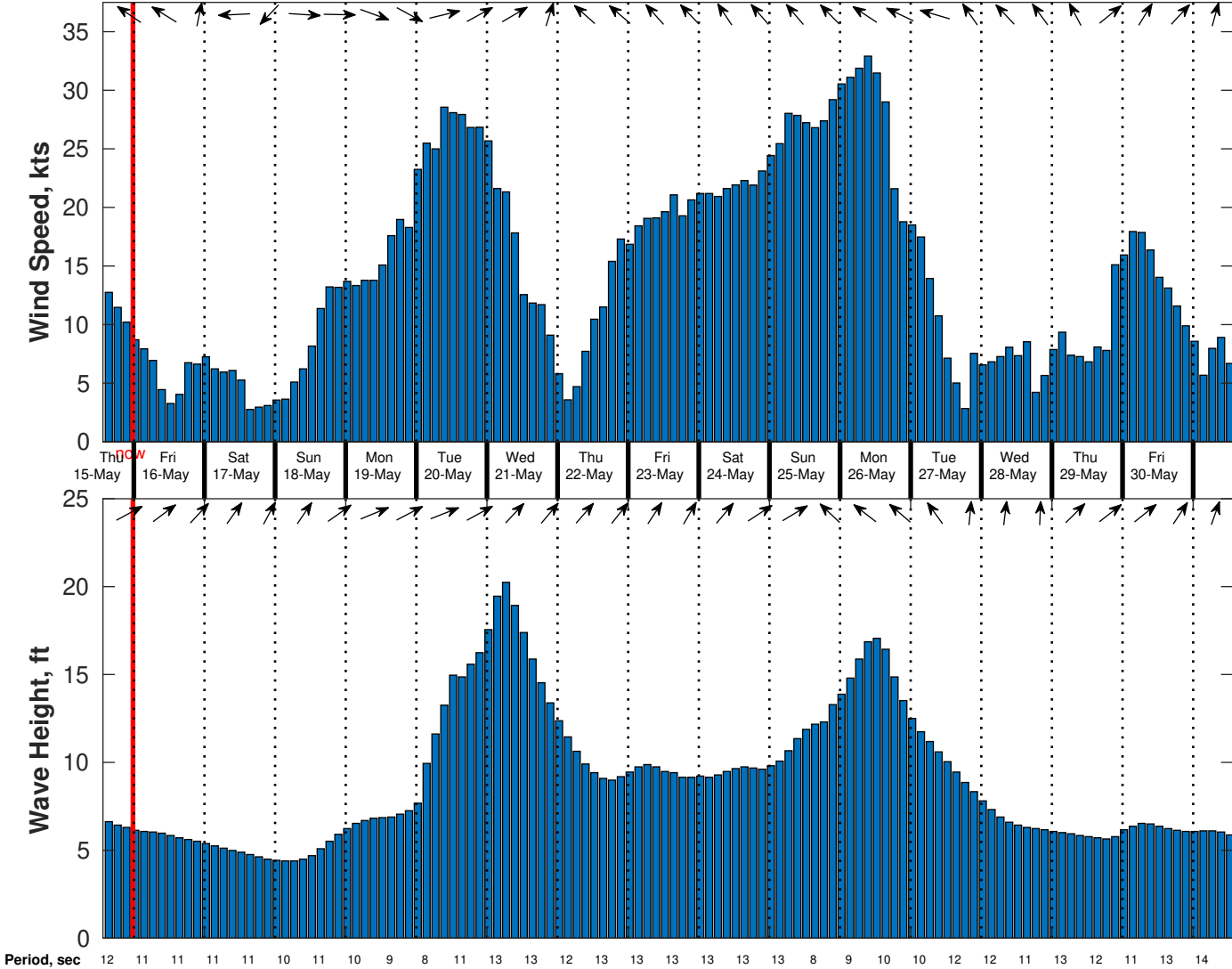
Wind & Wave Forecast for Benthic Solutions South Africa HF Site1 from 15-May-2025 14:00:00 to 31-May-2025 14:00:00
