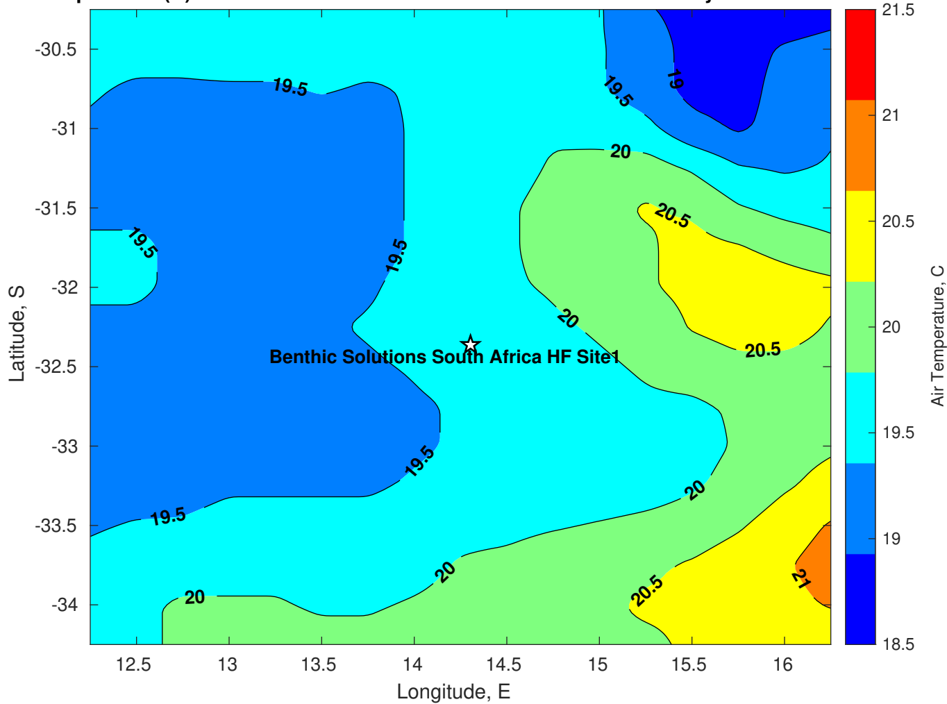
Air Temperature (C) for Benthic Solutions South Africa HF Site1 at 16-May-2025
