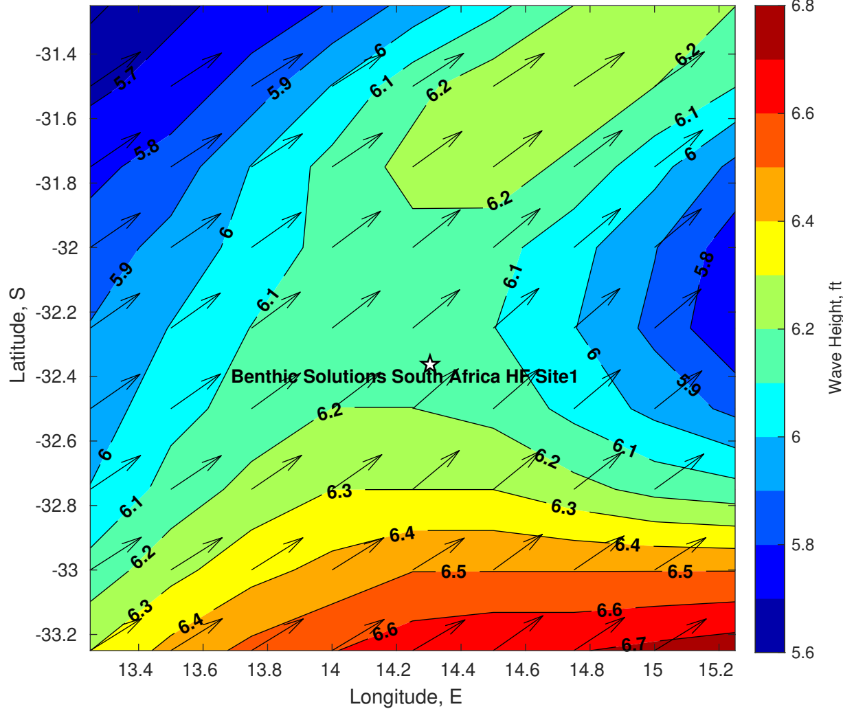
Wave Height (ft) for Benthic Solutions South Africa HF Site1 at 15-May-2025 21:00:00
