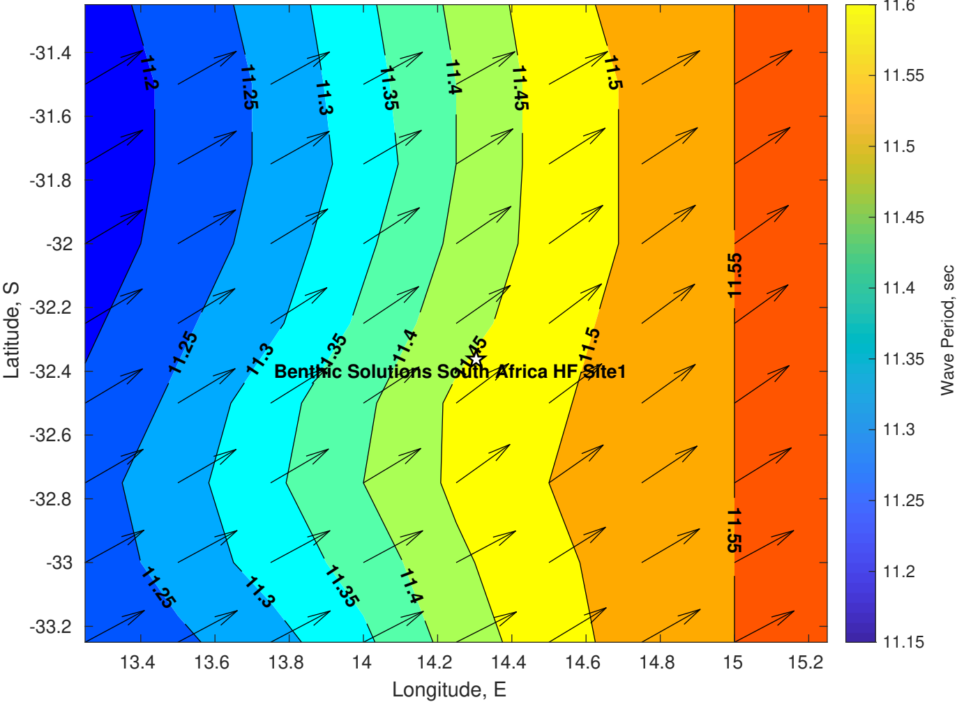
Wave Period (sec) for Benthic Solutions South Africa HF Site1 at 15-May-2025 21:00:00
