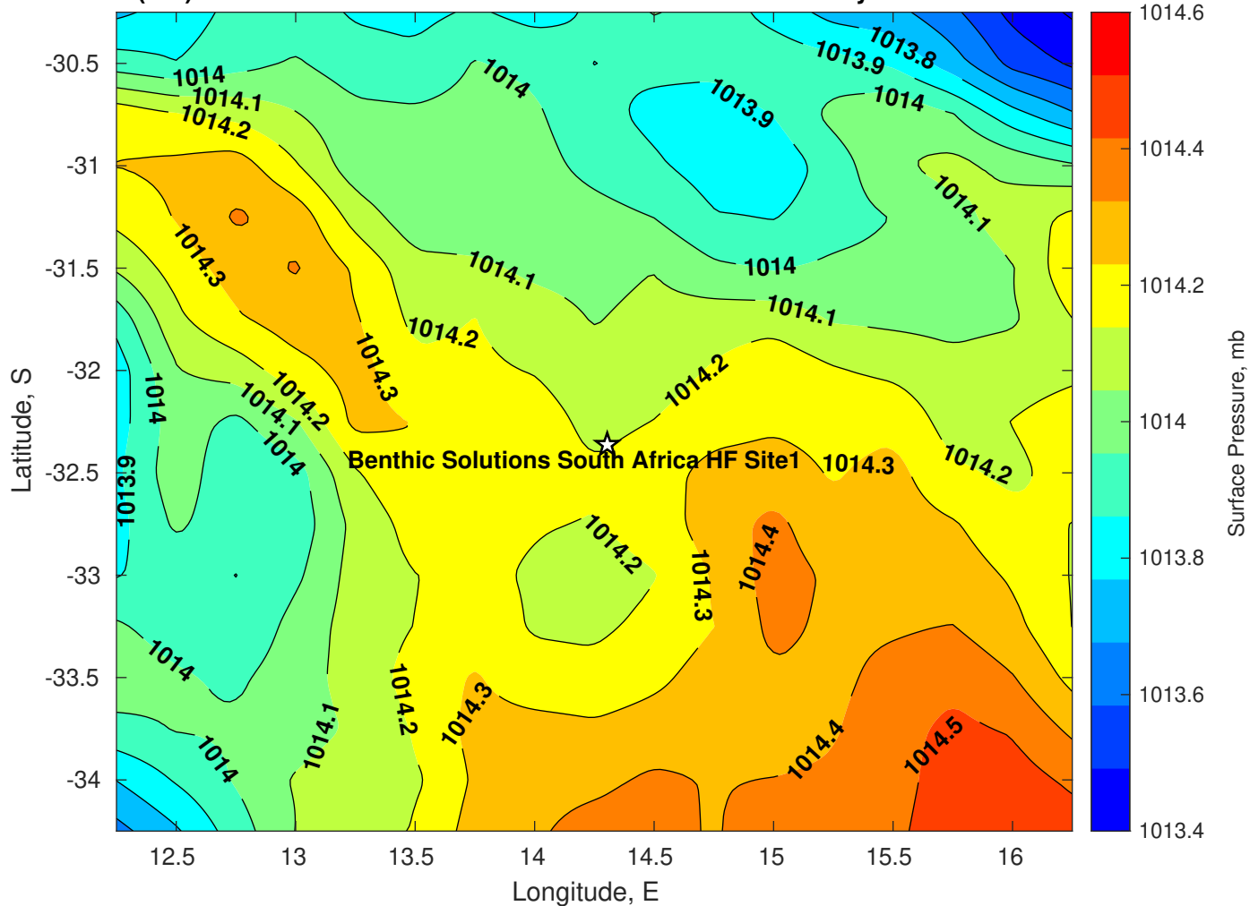
Surface Pressure (mb) for Benthic Solutions South Africa HF Site1 at 17-May-2025 00:00:00
