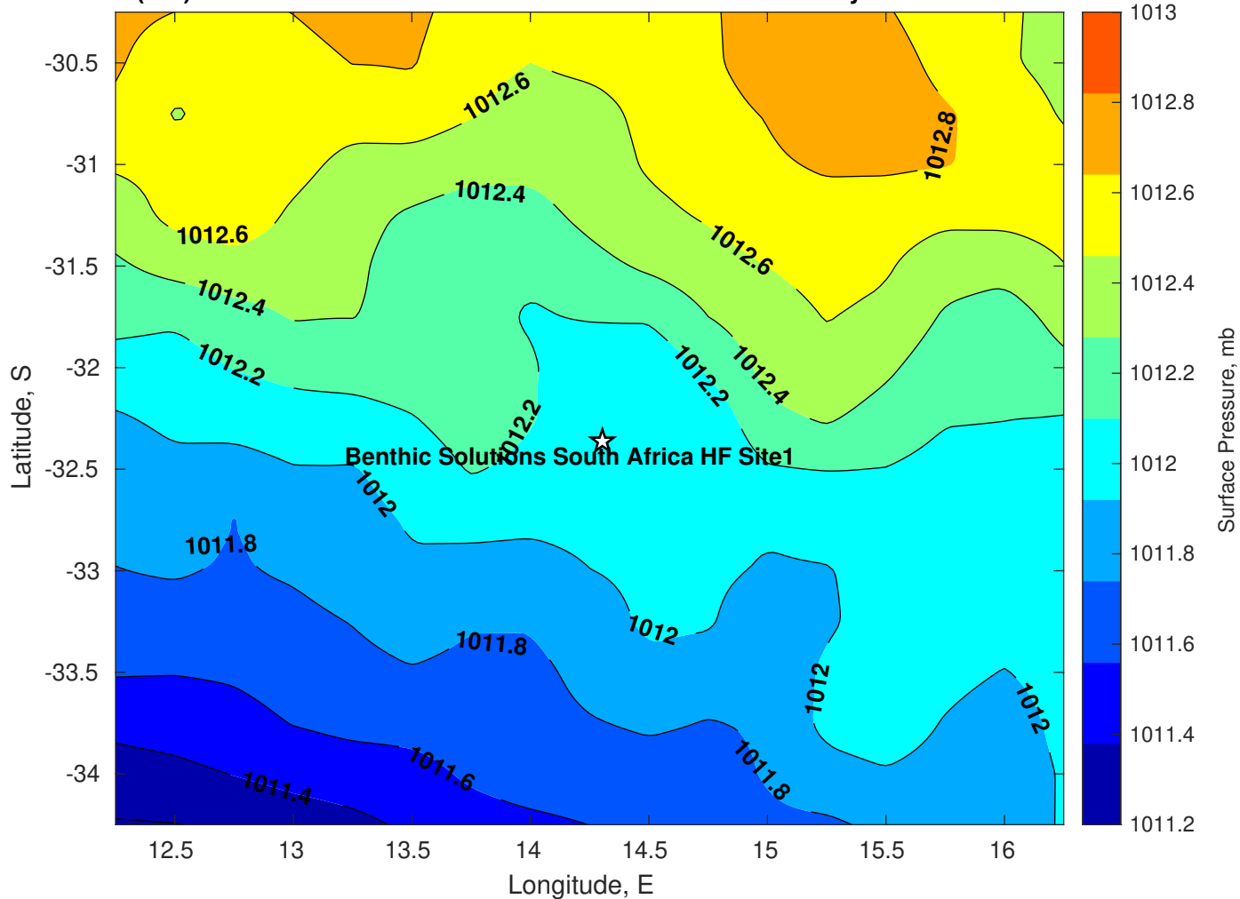
Surface Pressure (mb) for Benthic Solutions South Africa HF Site1 at 18-May-2025 00:00:00
