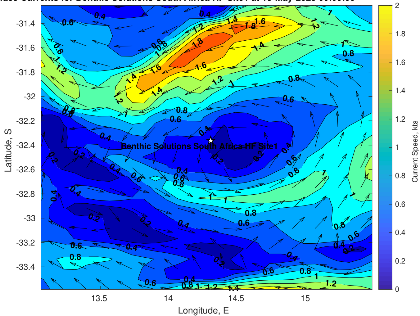
Surface Currents for Benthic Solutions South Africa HF Site1 at 15-May-2025 00:00:00
