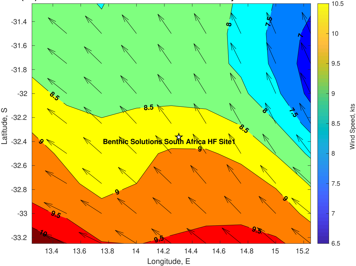
Winds (kts) for Benthic Solutions South Africa HF Site1 at 15-May-2025 21:00:00
