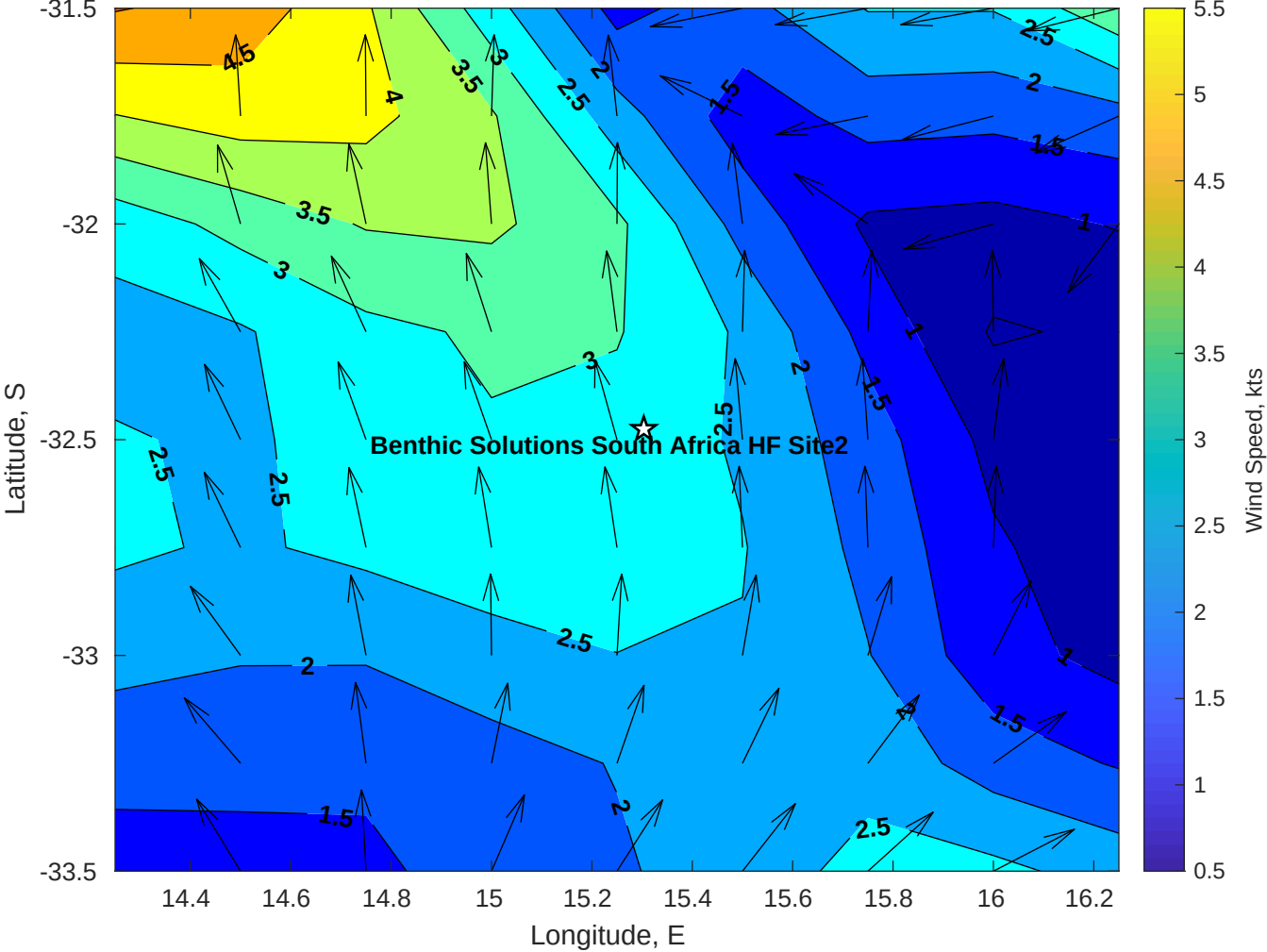
Winds (kts) for Benthic Solutions South Africa HF Site2 at 16-May-2025 09:00:00
