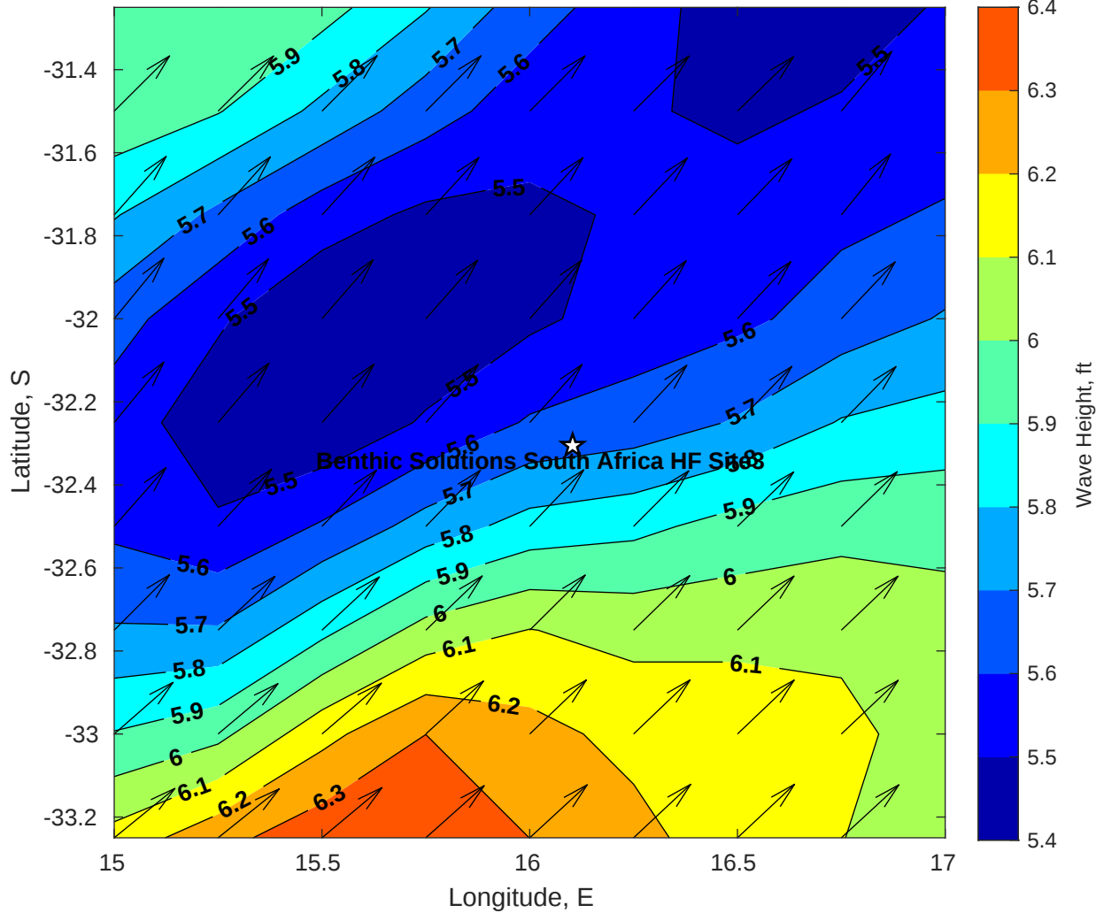
Wave Height (ft) for Benthic Solutions South Africa HF Site3 at 16-May-2025 09:00:00
