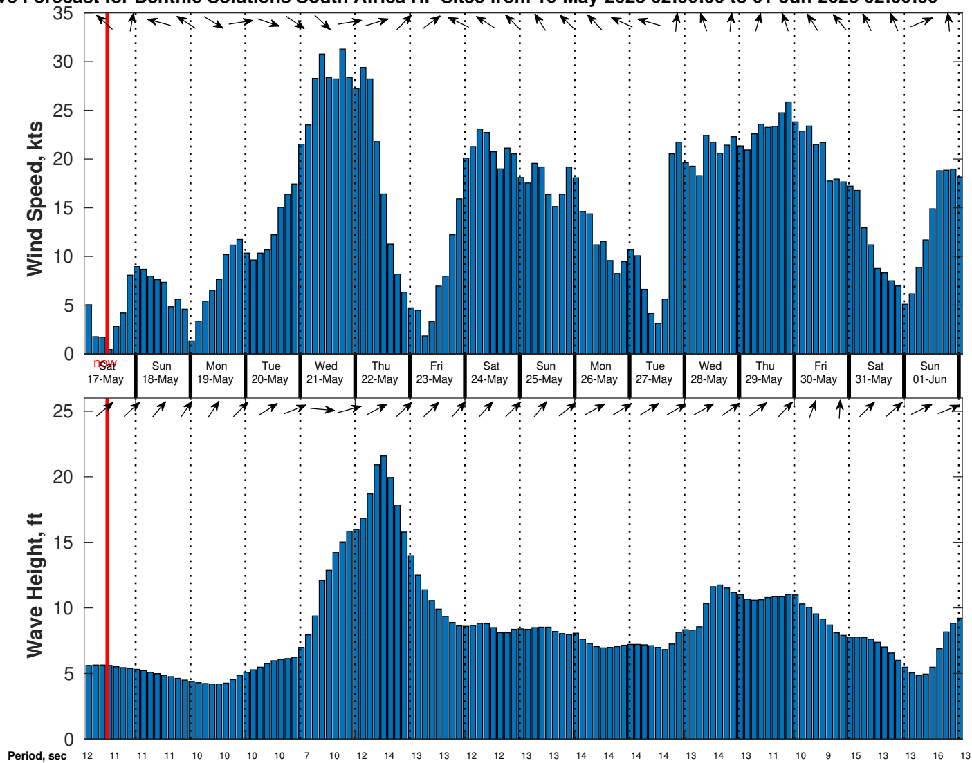
Wind & Wave Forecast for Benthic Solutions South Africa HF Site3 from 16-May-2025 02:00:00 to 01-Jun-2025 02:00:00
