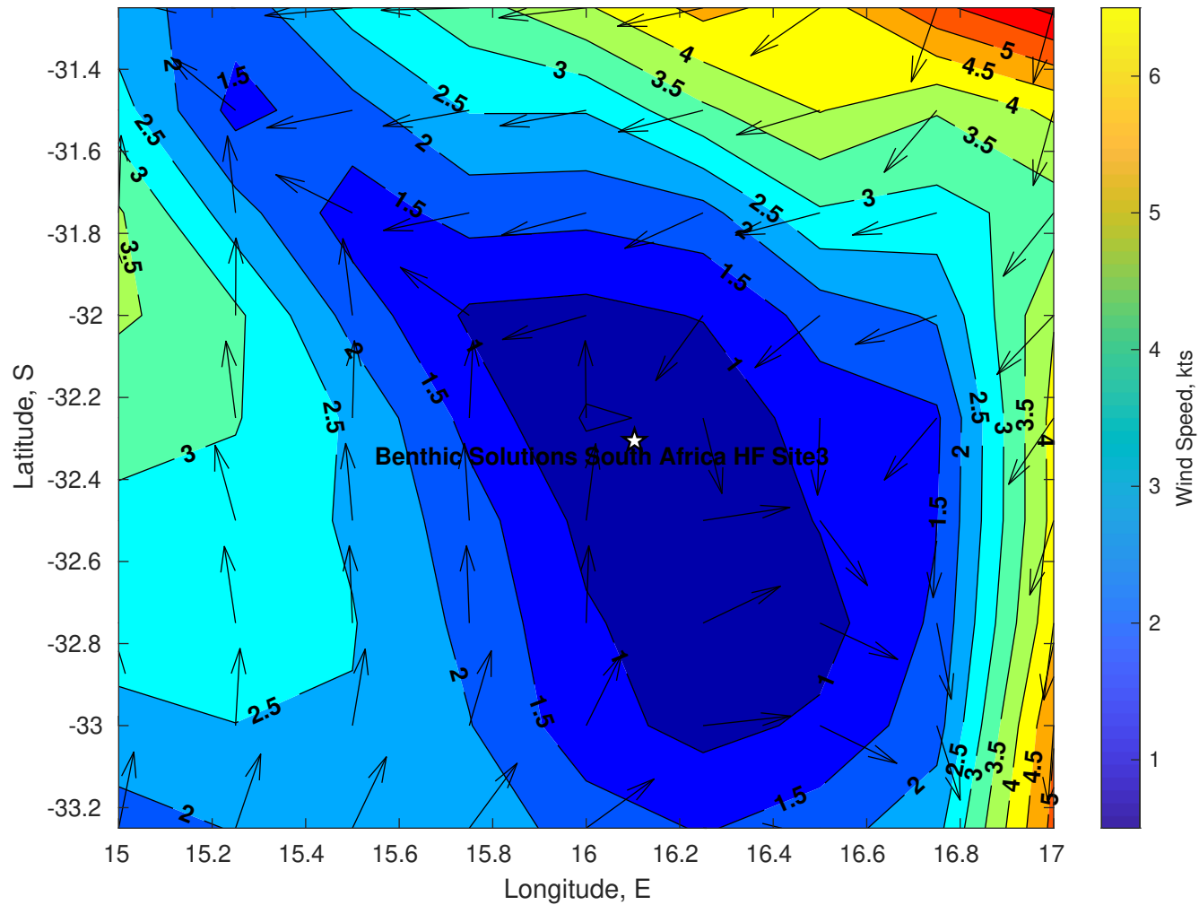
Winds (kts) for Benthic Solutions South Africa HF Site3 at 16-May-2025 09:00:00
