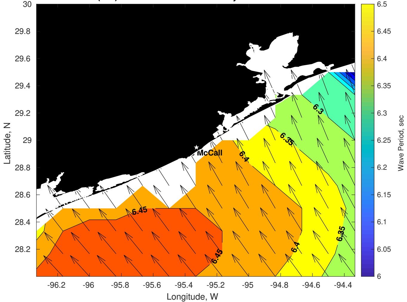
Wave Period (sec) for Brooks McCall at 16-May-2025 09:00:00
