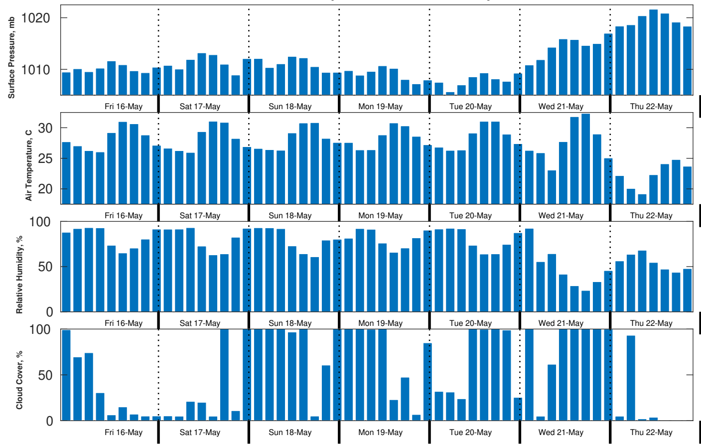
Met Forecast for Brooks McCall from 16-May-2025 00:00:00 to 23-May-2025 00:00:00
