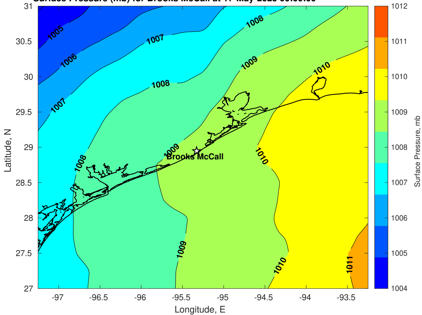
Surface Pressure (mb) for Brooks McCall at 17-May-2025 00:00:00
