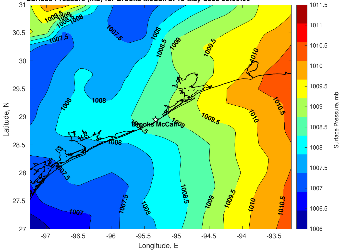
Surface Pressure (mb) for Brooks McCall at 18-May-2025 00:00:00
