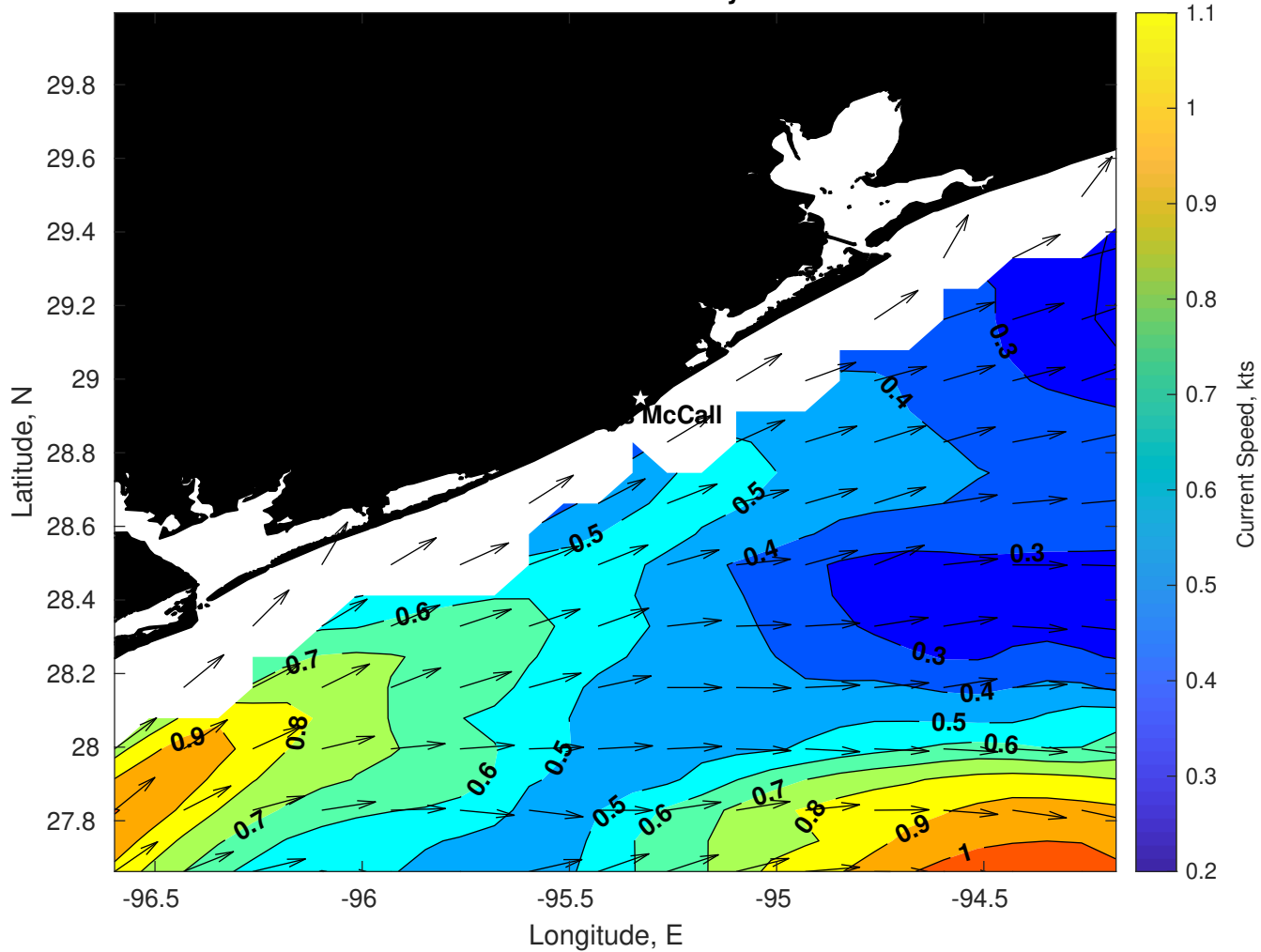
Surface Currents for Brooks McCall at 15-May-2025 00:00:00
