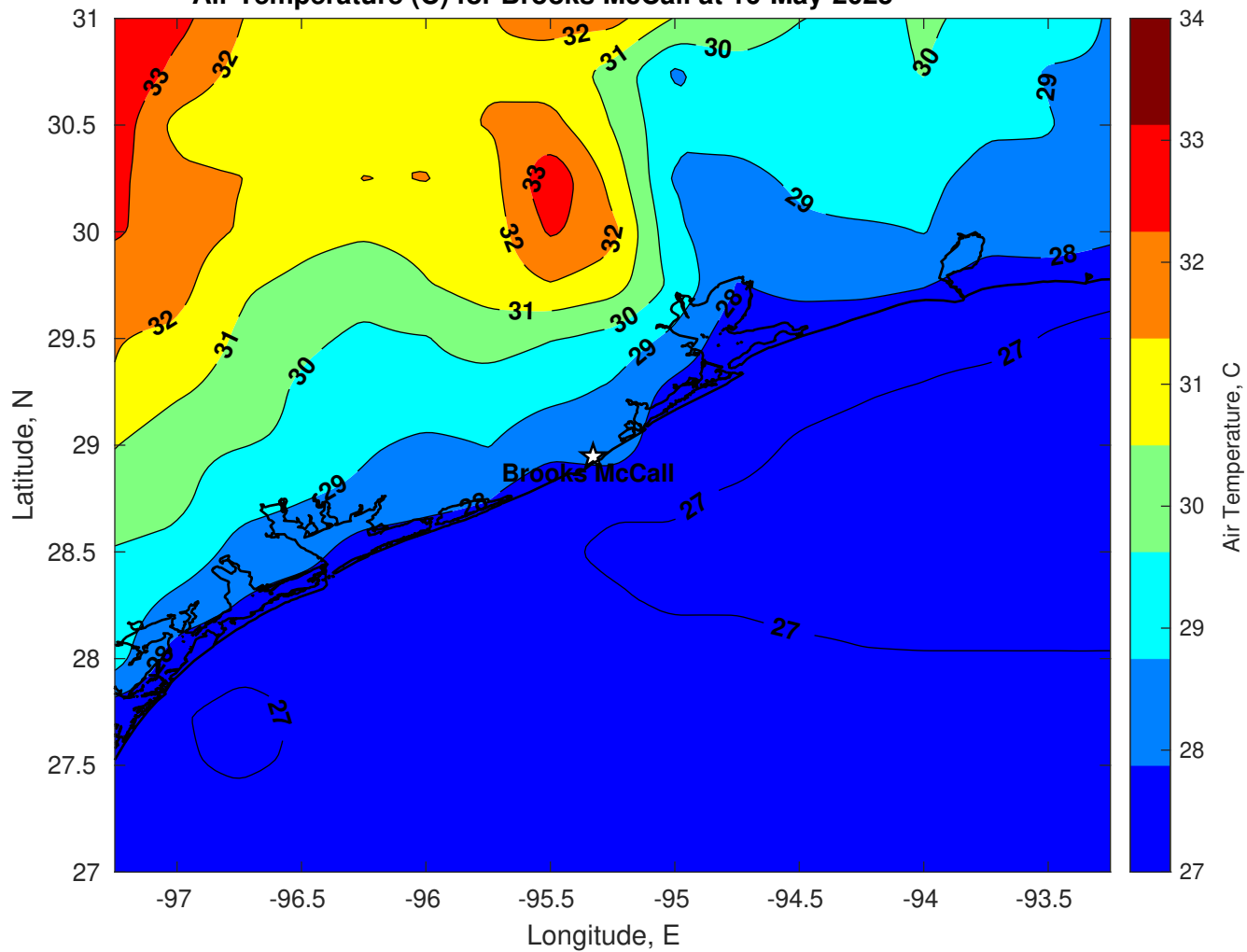
Air Temperature (C) for Brooks McCall at 16-May-2025
