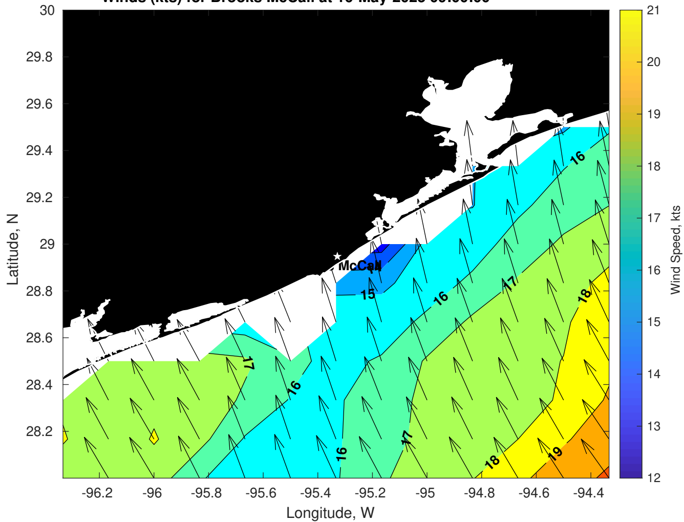
Winds (kts) for Brooks McCall at 16-May-2025 09:00:00
