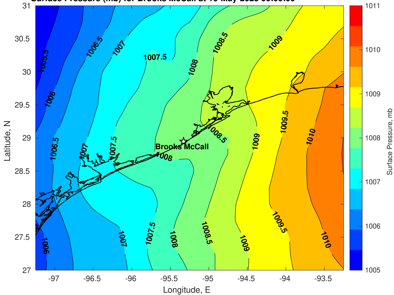
Surface Pressure (mb) for Brooks McCall at 16-May-2025 00:00:00
