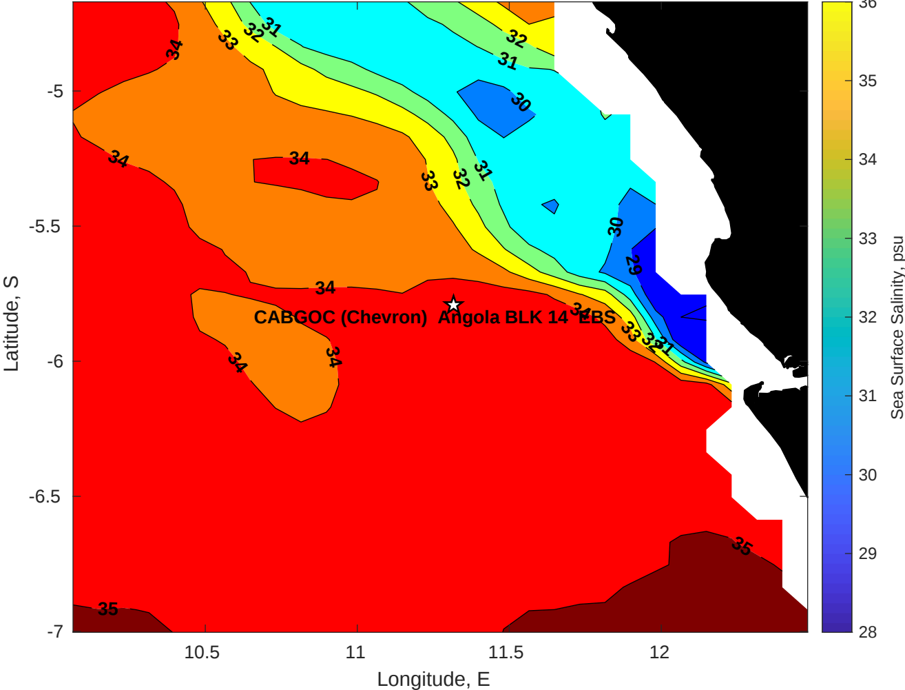
Surface Salinity for CABGOC (Chevron) Angola BLK 14 EBS at 15-May-2025 00:00:00
