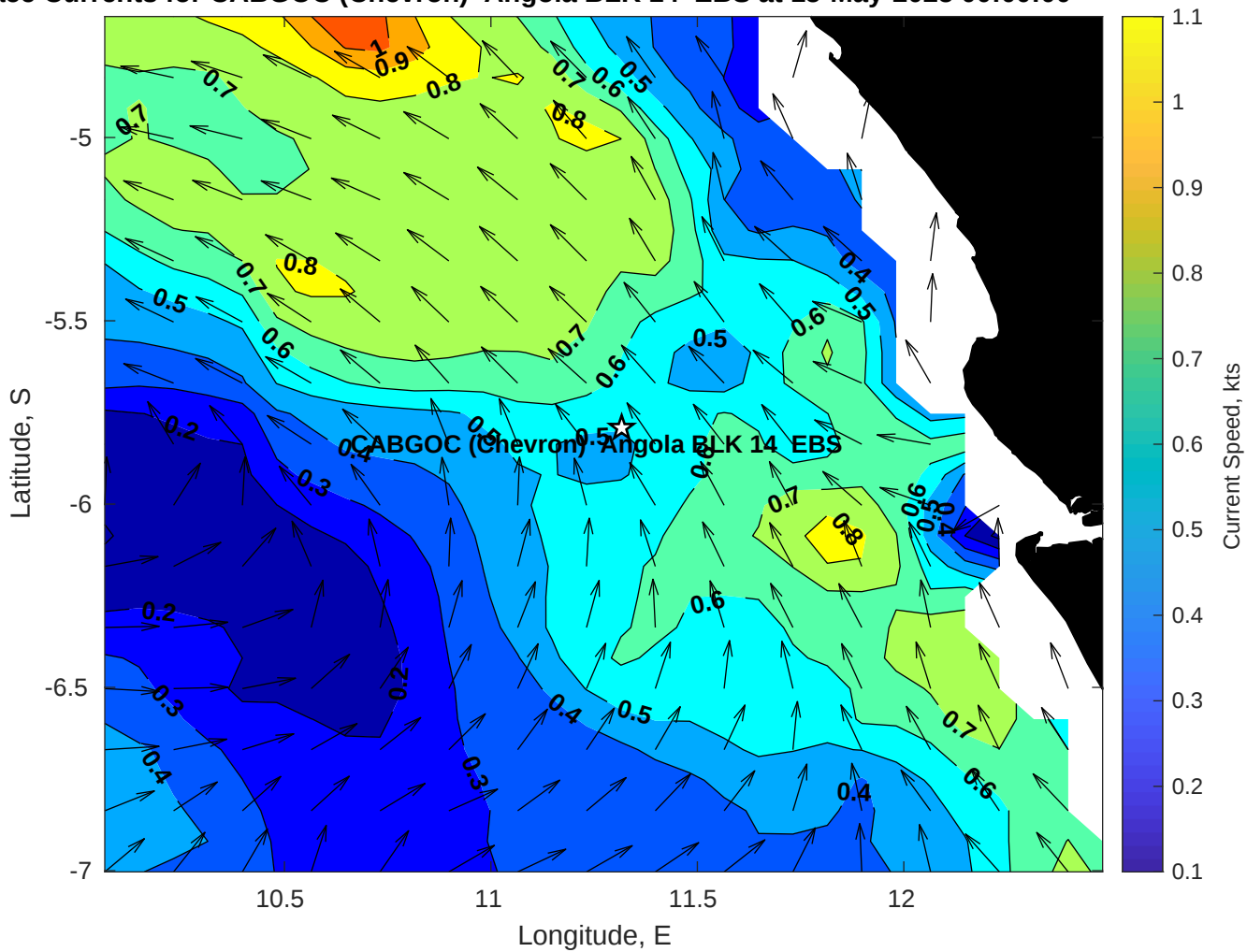
Surface Currents for CABGOC (Chevron) Angola BLK 14 EBS at 15-May-2025 00:00:00
