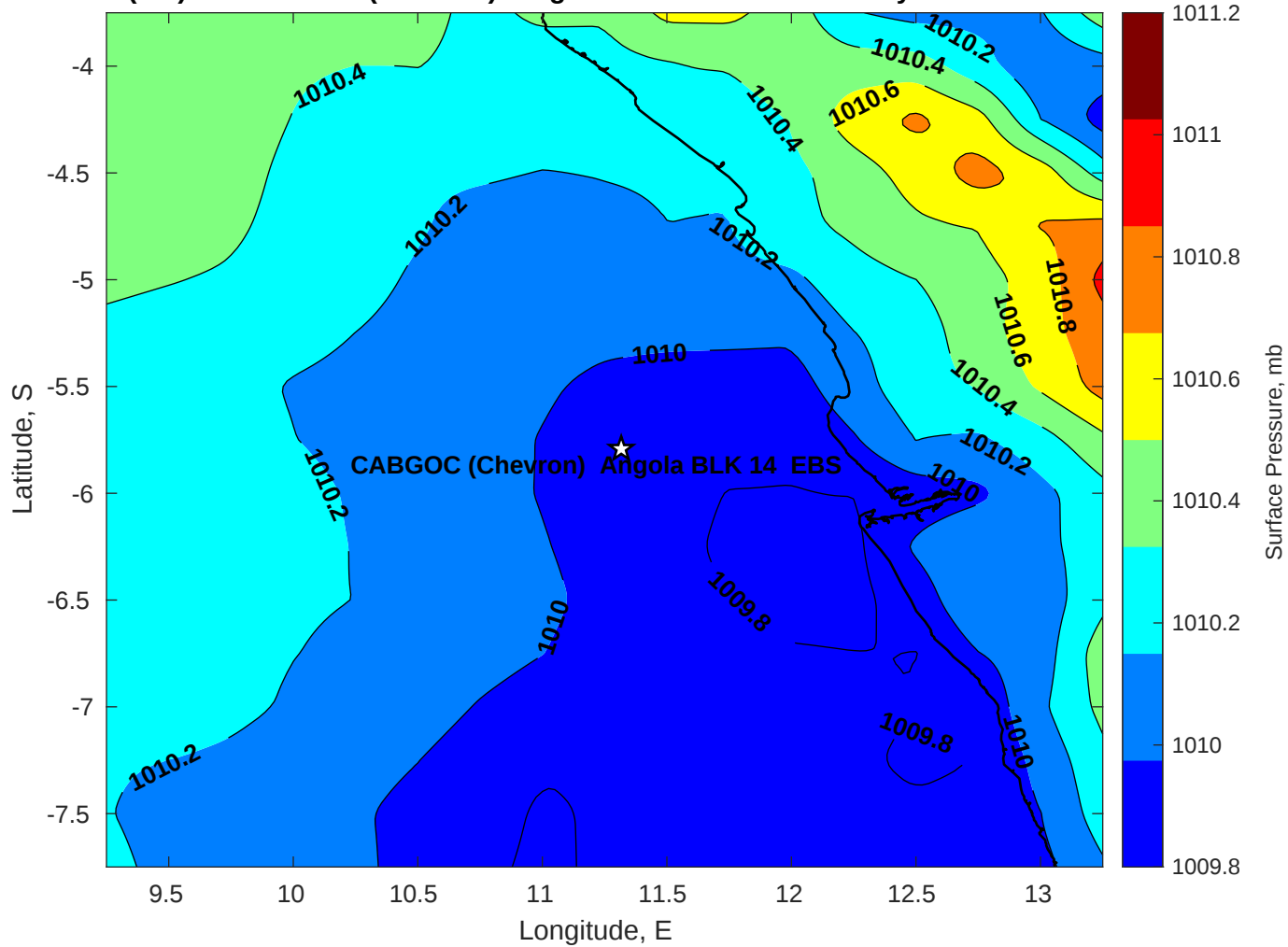
Surface Pressure (mb) for CABGOC (Chevron) Angola BLK 14 EBS at 16-May-2025 00:00:00
