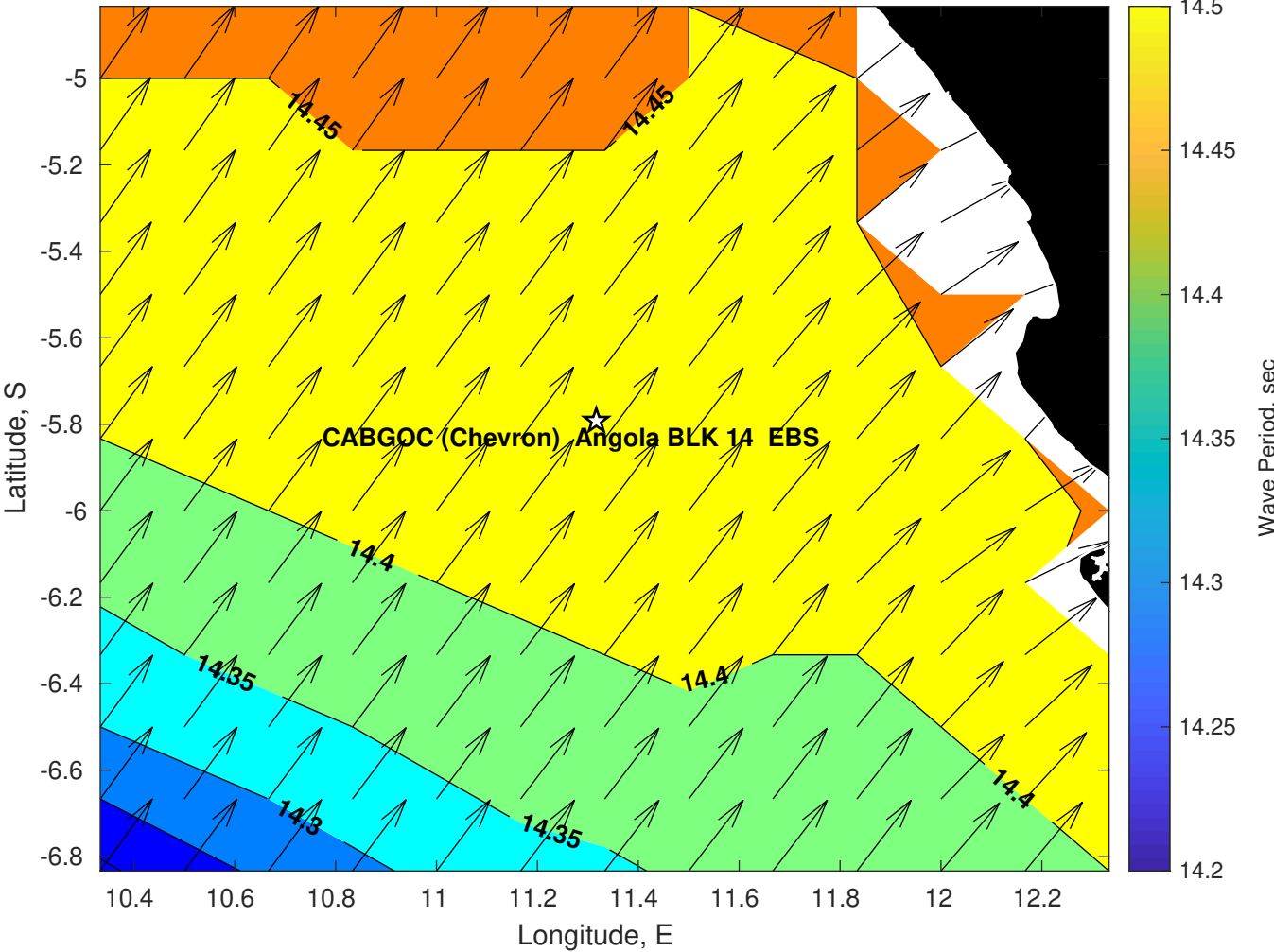
Wave Period (sec) for CABGOC (Chevron) Angola BLK 14 EBS at 16-May-2025 09:00:00
