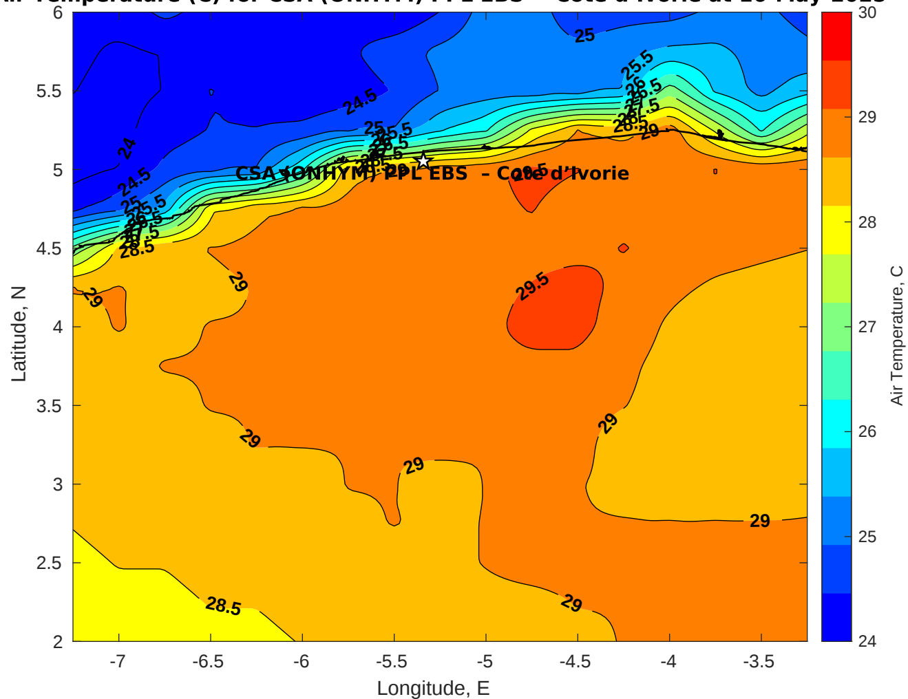
Air Temperature (C) for CSA (ONHYM) PPL EBS - Cote d'Ivoire at 16-May-2025
