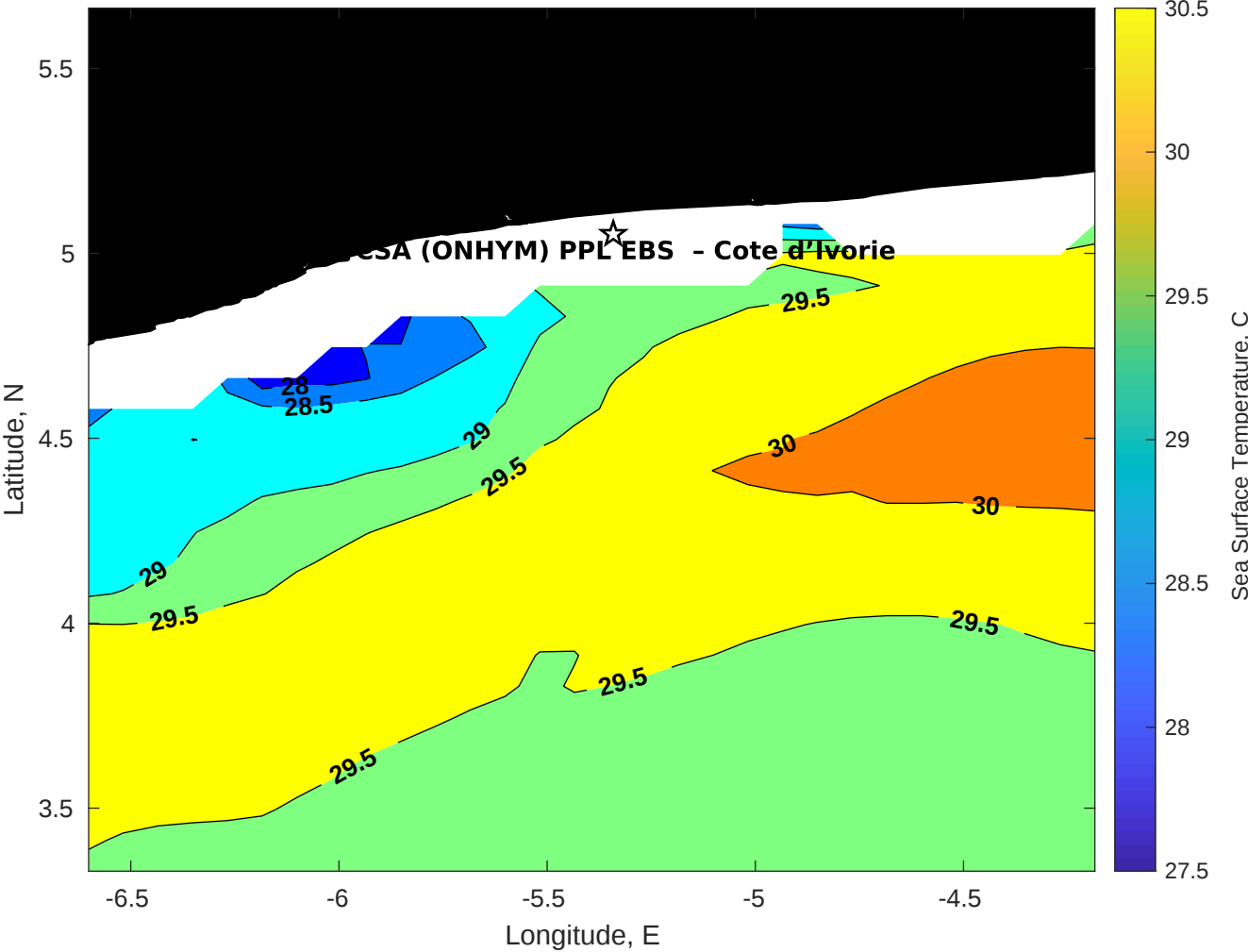
SST for CSA (ONHYM) PPL EBS - Cote d'Ivoire at 15-May-2025 00:00:00
