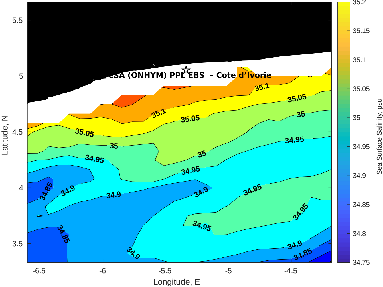
Surface Salinity for CSA (ONHYM) PPL EBS - Cote d'Ivoire at 15-May-2025 00:00:00
